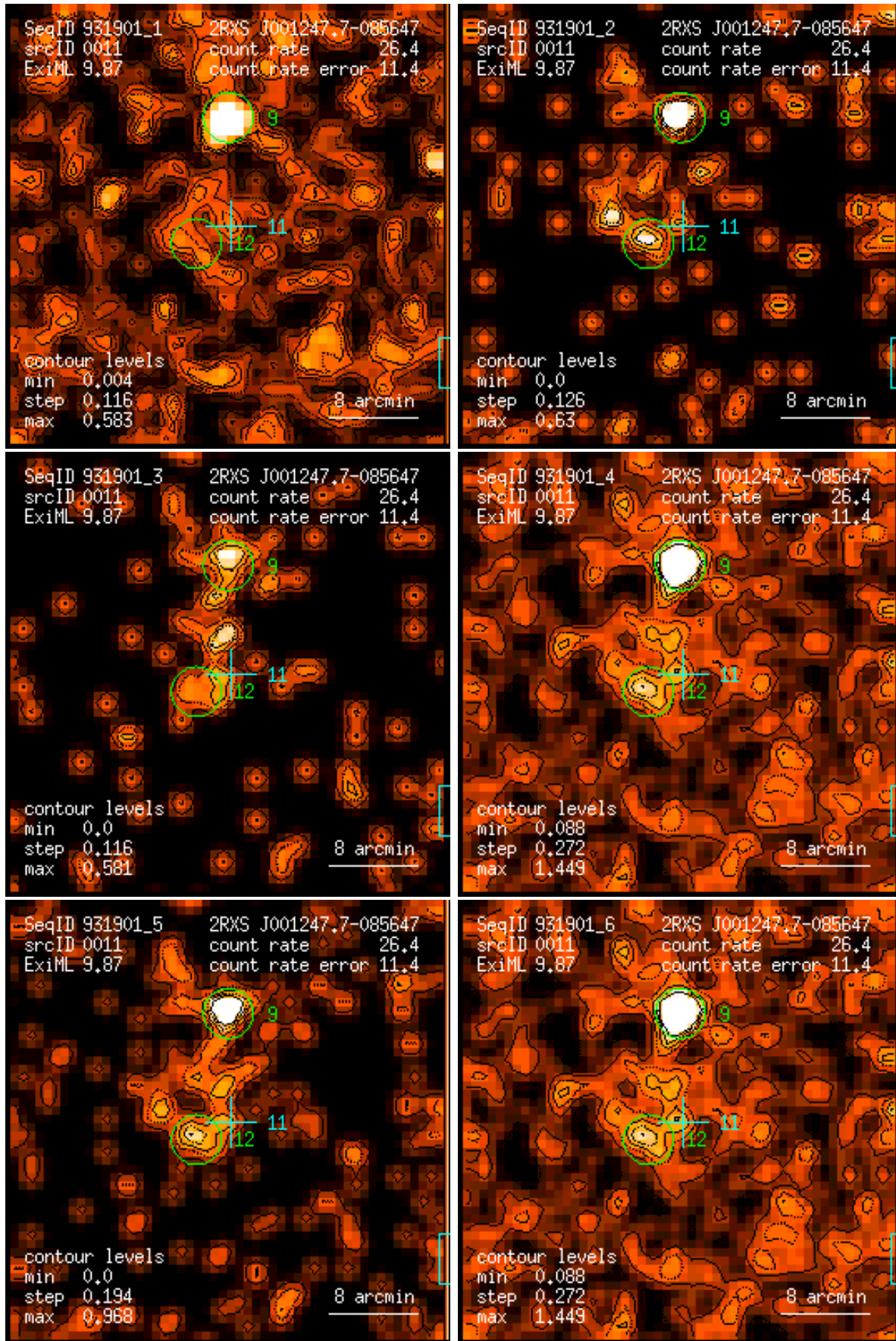
Figure 11: RASS 931901: detection 0011: band rate images, Gaussian filter: (1) PSPC channels 11 – 41, (2) 52 – 90, (3) 91 – 201, (4) 11 – 235, (5) 52 – 201, (6) 11 – 201. Broad band rates in counts/ks. Band rate contour levels in counts/ks/arcmin 2 .
