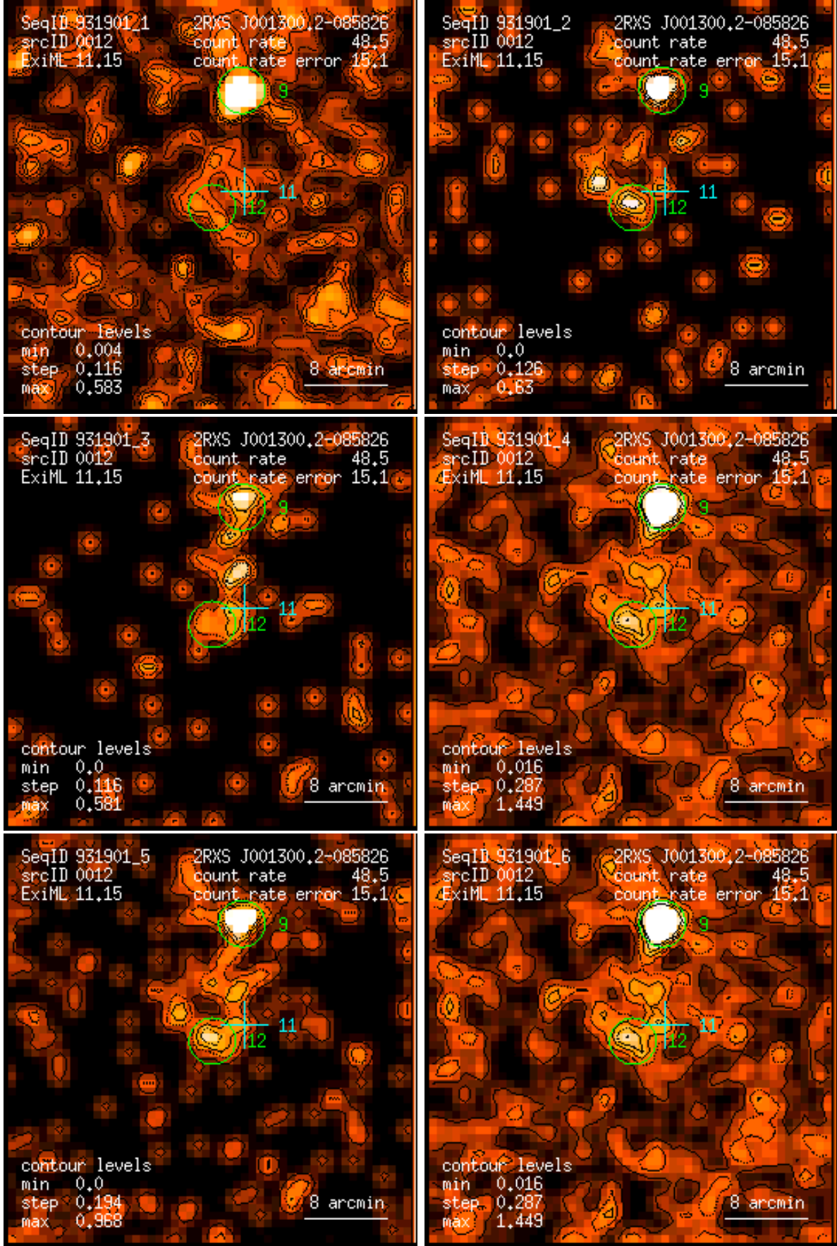
Figure 12: RASS 931901: detection 0012: band rate images, Gaussian filter: (1) PSPC channels 11 – 41, (2) 52 – 90, (3) 91 – 201, (4) 11 – 235, (5) 52 – 201, (6) 11 – 201. Broad band rates in counts/ks. Band rate contour levels in counts/ks/arcmin 2 .
