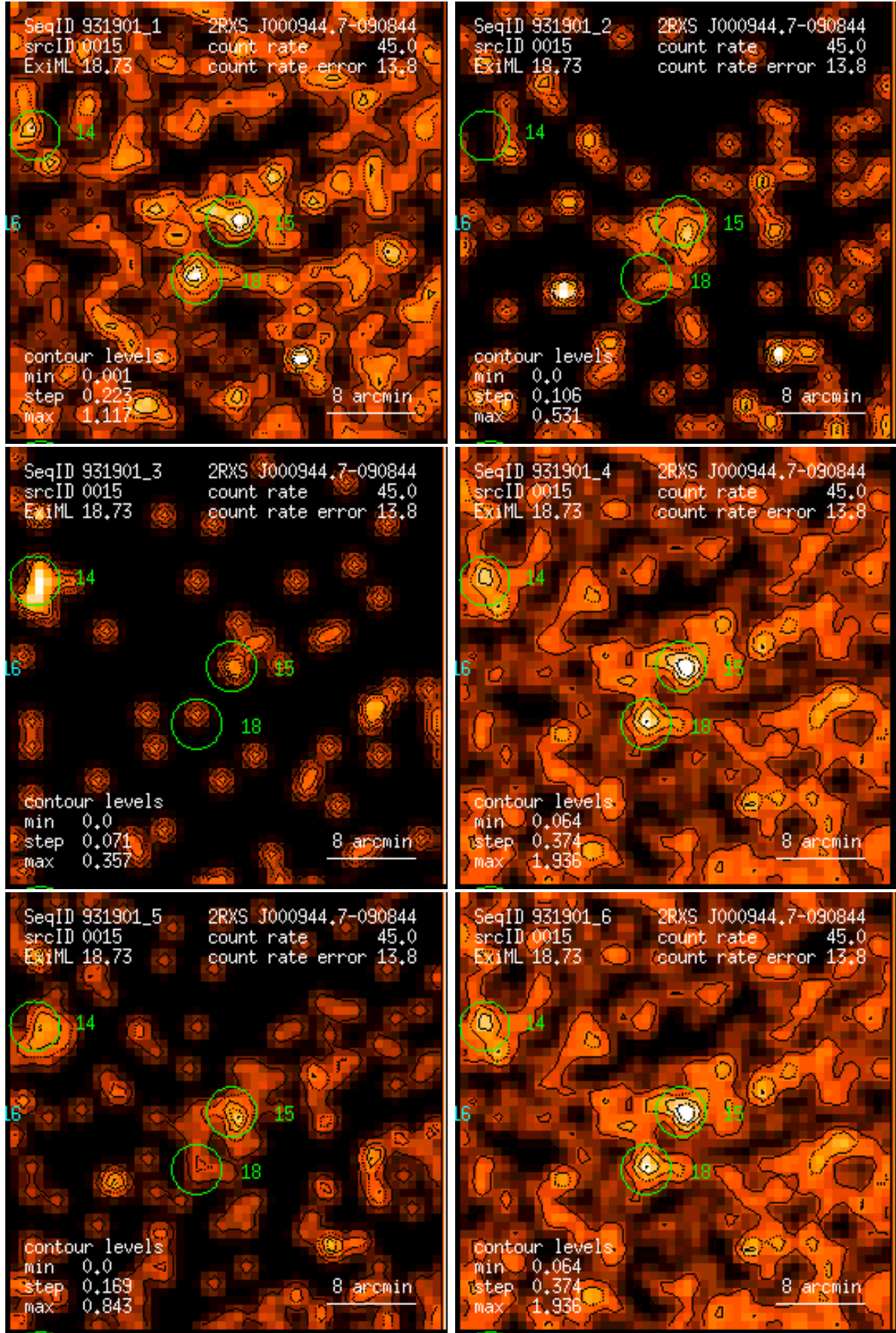
Figure 15: RASS 931901: detection 0015: band rate images, Gaussian filter: (1) PSPC channels 11 – 41, (2) 52 – 90, (3) 91 – 201, (4) 11 – 235, (5) 52 – 201, (6) 11 – 201. Broad band rates in counts/ks. Band rate contour levels in counts/ks/arcmin 2 .
