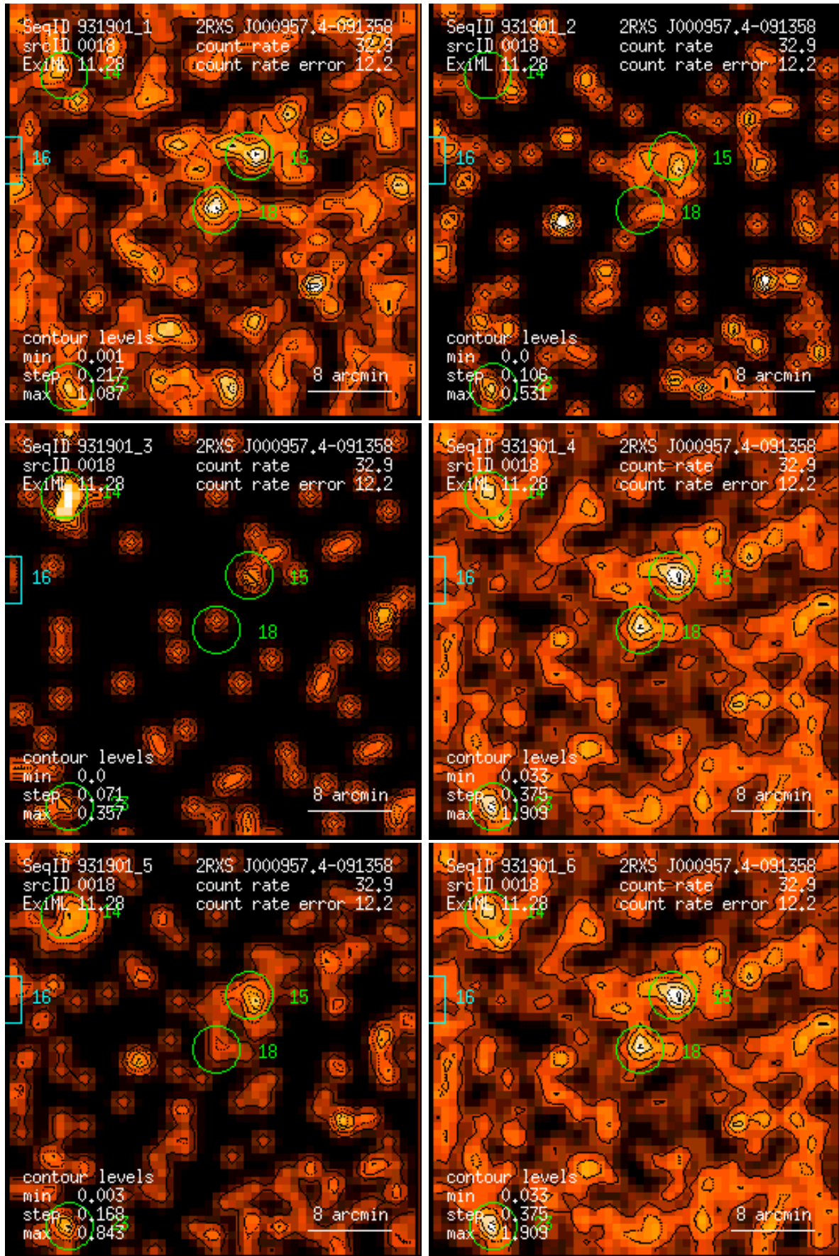
Figure 18: RASS 931901: detection 0018: band rate images, Gaussian filter: (1) PSPC channels 11 – 41, (2) 52 – 90, (3) 91 – 201, (4) 11 – 235, (5) 52 – 201, (6) 11 – 201. Broad band rates in counts/ks. Band rate contour levels in counts/ks/arcmin 2 .
