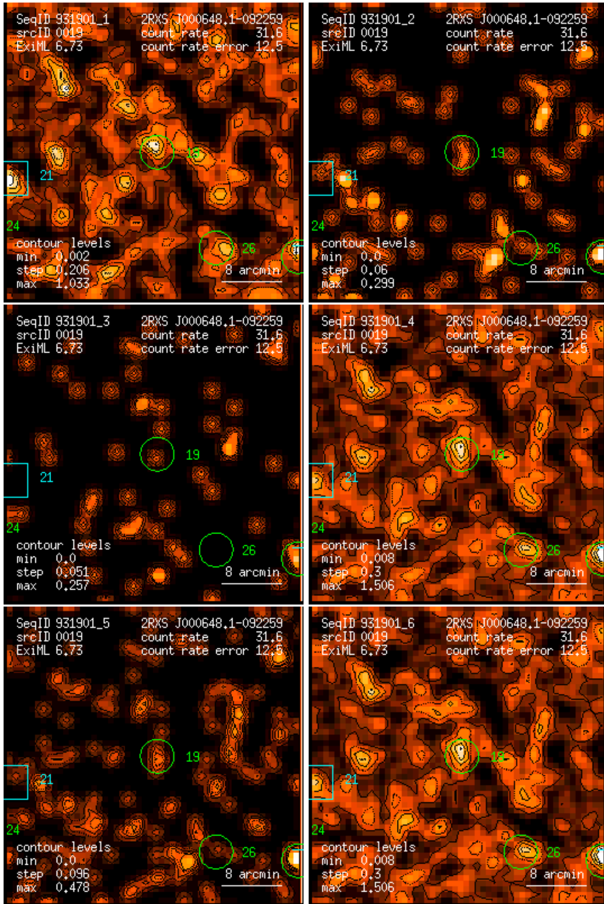
Figure 19: RASS 931901: detection 0019: band rate images, Gaussian filter: (1) PSPC channels 11 – 41, (2) 52 – 90, (3) 91 – 201, (4) 11 – 235, (5) 52 – 201, (6) 11 – 201. Broad band rates in counts/ks. Band rate contour levels in counts/ks/arcmin 2 .
