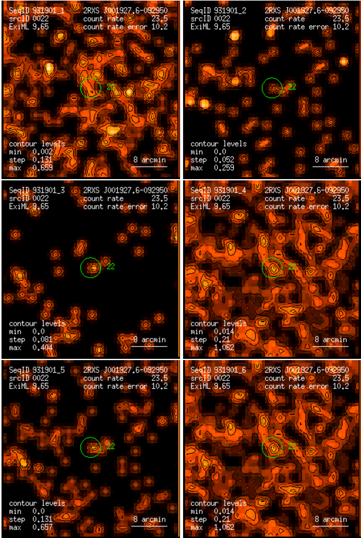
Figure 22: RASS 931901: detection 0022: band rate images, Gaussian filter: (1) PSPC channels 11 – 41, (2) 52 – 90, (3) 91 – 201, (4) 11 – 235, (5) 52 – 201, (6) 11 – 201. Broad band rates in counts/ks. Band rate contour levels in counts/ks/arcmin 2 .
