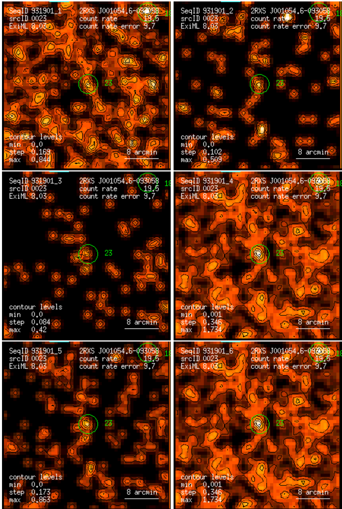
Figure 23: RASS 931901: detection 0023: band rate images, Gaussian filter: (1) PSPC channels 11 – 41, (2) 52 – 90, (3) 91 – 201, (4) 11 – 235, (5) 52 – 201, (6) 11 – 201. Broad band rates in counts/ks. Band rate contour levels in counts/ks/arcmin 2 .
