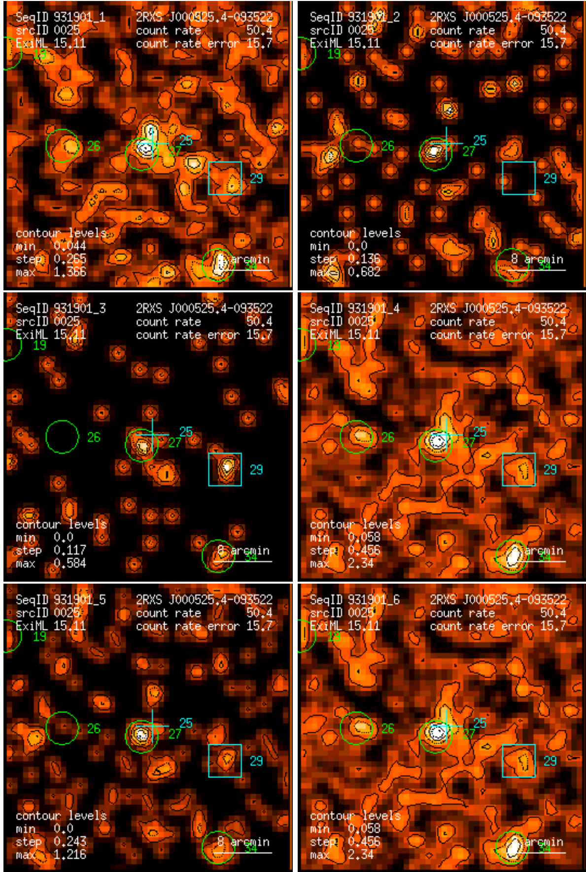
Figure 25: RASS 931901: detection 0025: band rate images, Gaussian filter: (1) PSPC channels 11 – 41, (2) 52 – 90, (3) 91 – 201, (4) 11 – 235, (5) 52 – 201, (6) 11 – 201. Broad band rates in counts/ks. Band rate contour levels in counts/ks/arcmin 2 .
