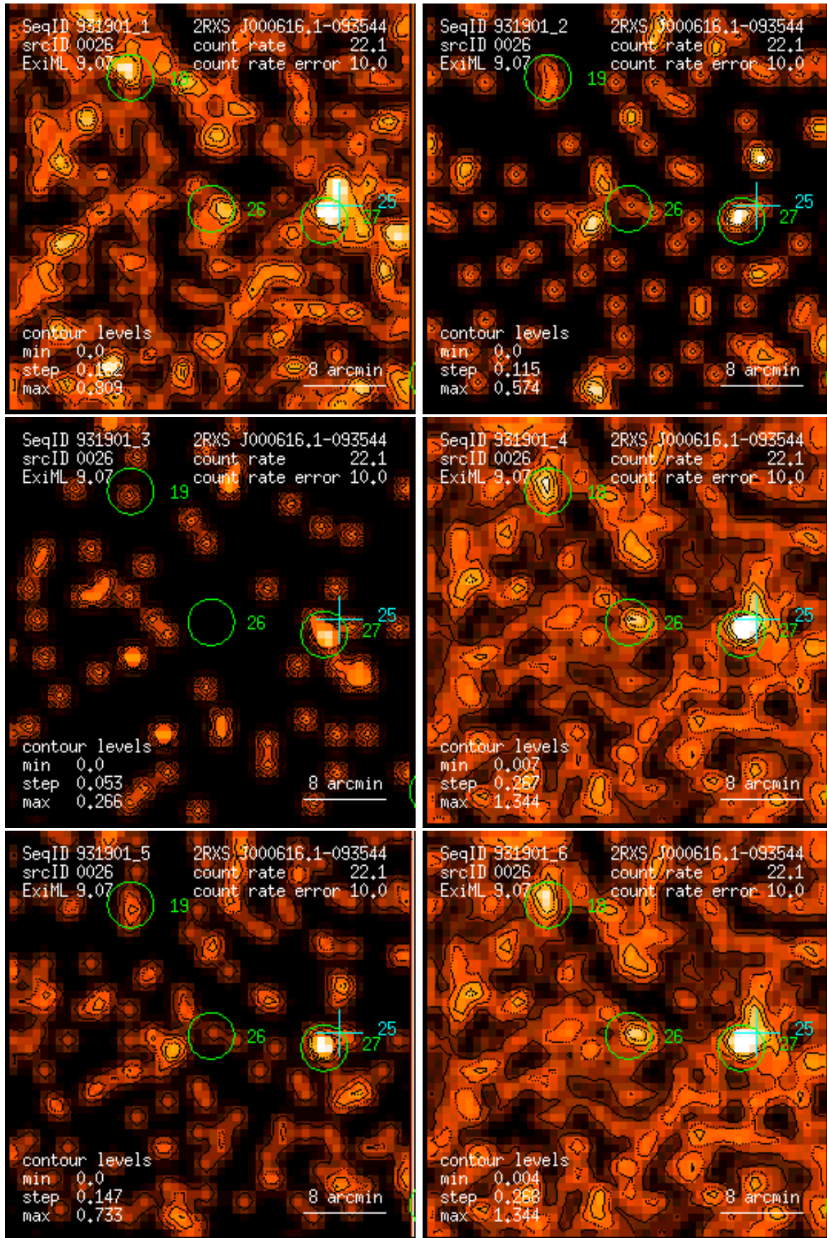
Figure 26: RASS 931901: detection 0026: band rate images, Gaussian filter: (1) PSPC channels 11 – 41, (2) 52 – 90, (3) 91 – 201, (4) 11 – 235, (5) 52 – 201, (6) 11 – 201. Broad band rates in counts/ks. Band rate contour levels in counts/ks/arcmin 2 .
