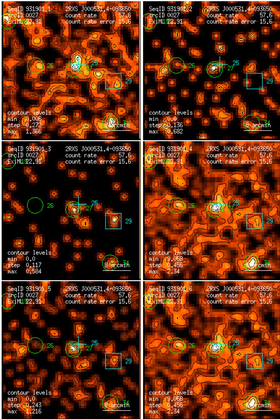
Figure 27: RASS 931901: detection 0027: band rate images, Gaussian filter: (1) PSPC channels 11 – 41, (2) 52 – 90, (3) 91 – 201, (4) 11 – 235, (5) 52 – 201, (6) 11 – 201. Broad band rates in counts/ks. Band rate contour levels in counts/ks/arcmin 2 .
