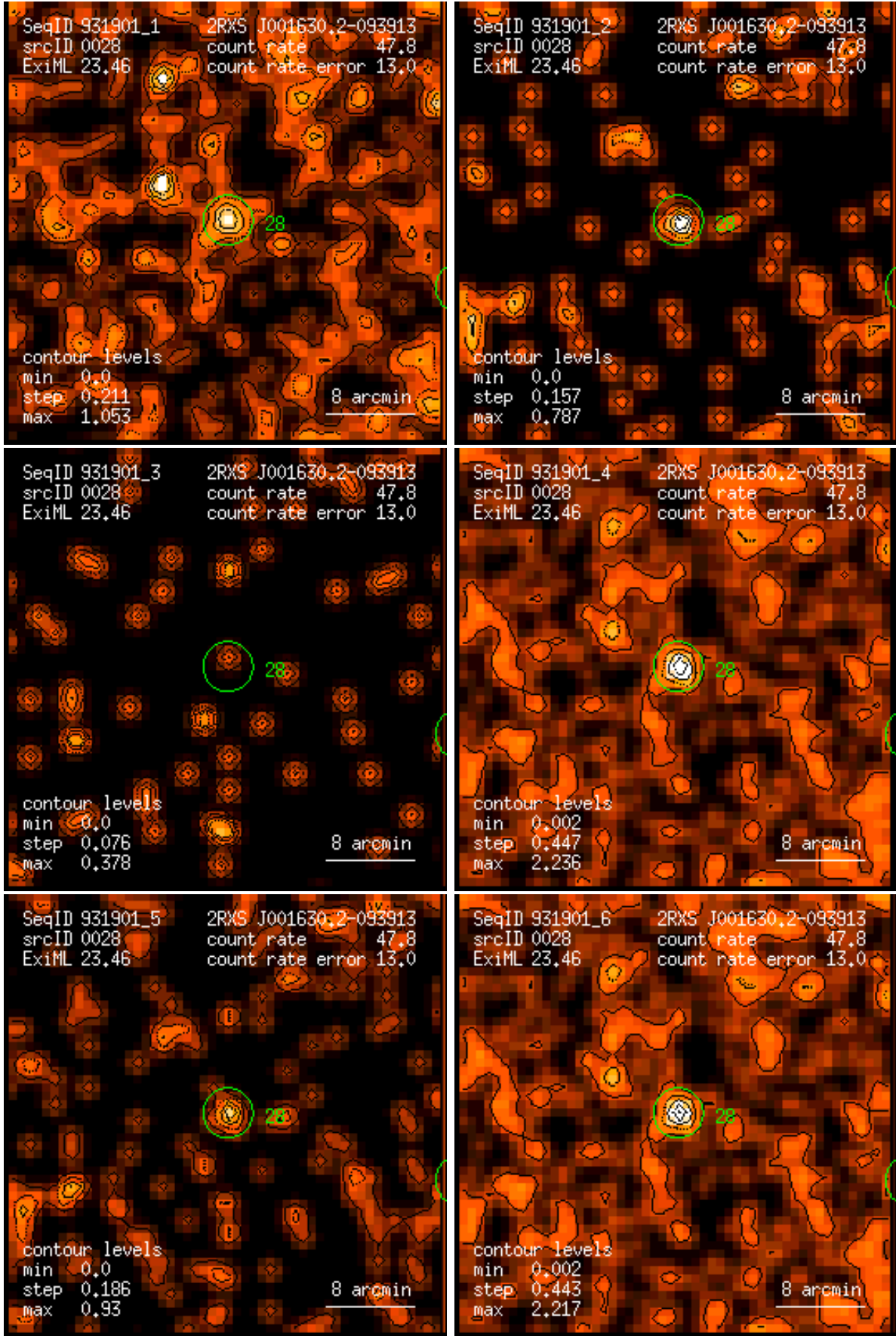
Figure 28: RASS 931901: detection 0028: band rate images, Gaussian filter: (1) PSPC channels 11 – 41, (2) 52 – 90, (3) 91 – 201, (4) 11 – 235, (5) 52 – 201, (6) 11 – 201. Broad band rates in counts/ks. Band rate contour levels in counts/ks/arcmin 2 .
