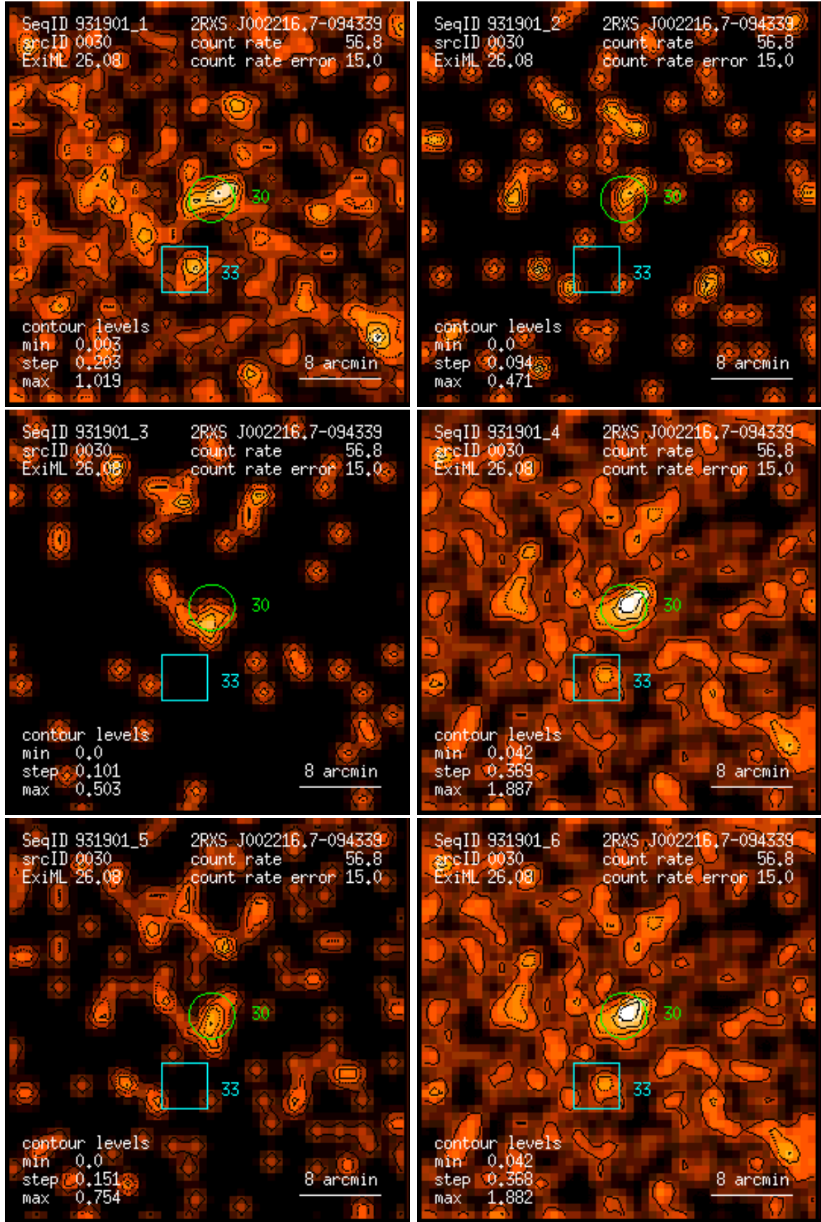
Figure 30: RASS 931901: detection 0030: band rate images, Gaussian filter: (1) PSPC channels 11 – 41, (2) 52 – 90, (3) 91 – 201, (4) 11 – 235, (5) 52 – 201, (6) 11 – 201. Broad band rates in counts/ks. Band rate contour levels in counts/ks/arcmin 2 .
