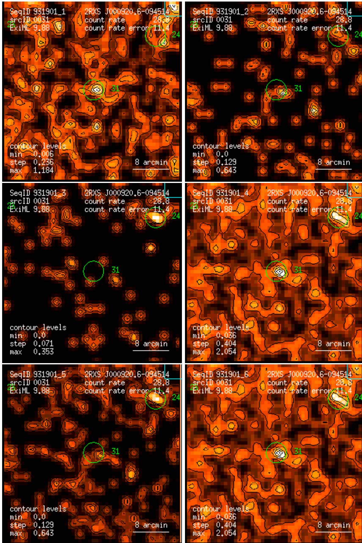
Figure 31: RASS 931901: detection 0031: band rate images, Gaussian filter: (1) PSPC channels 11 – 41, (2) 52 – 90, (3) 91 – 201, (4) 11 – 235, (5) 52 – 201, (6) 11 – 201. Broad band rates in counts/ks. Band rate contour levels in counts/ks/arcmin 2 .
