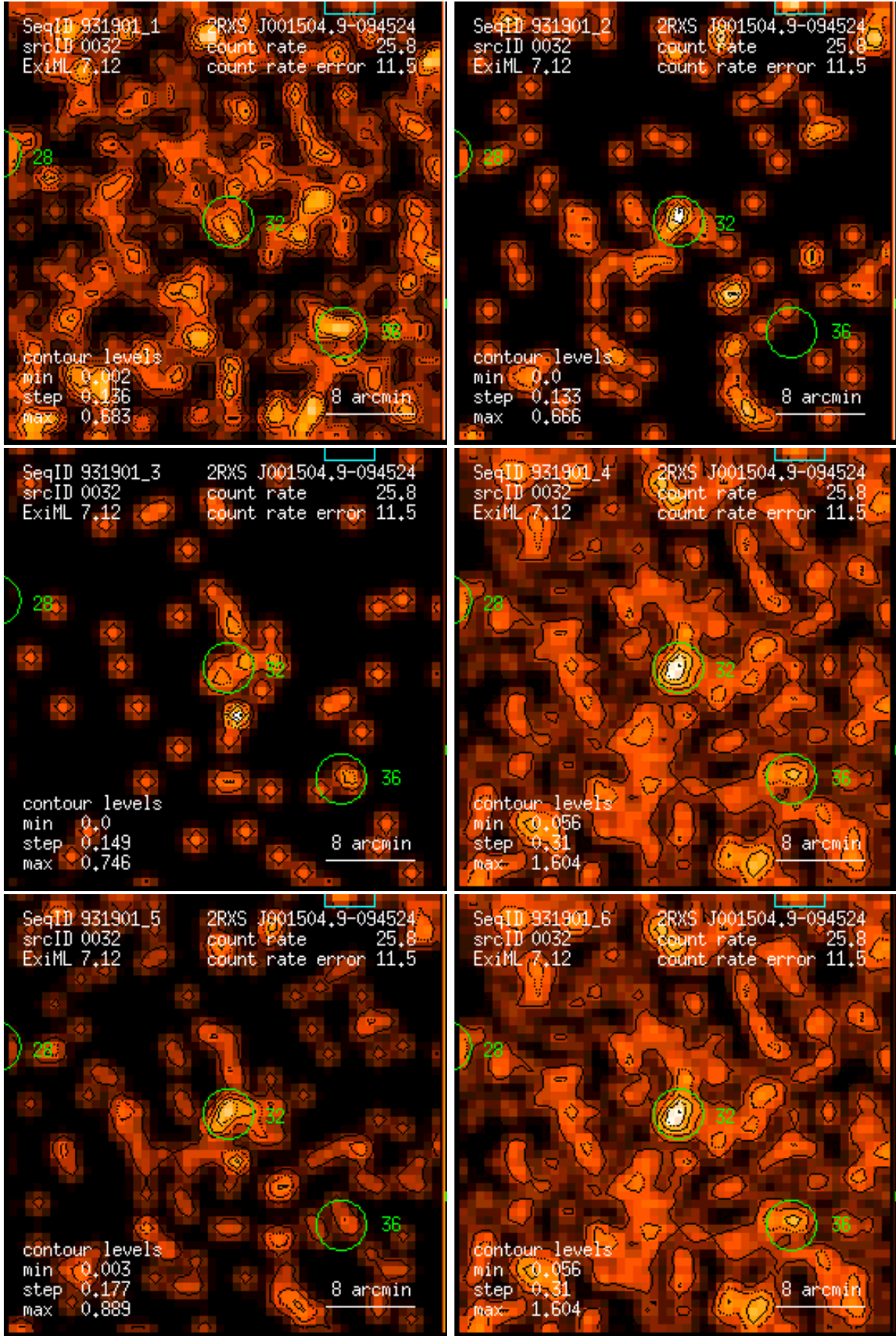
Figure 32: RASS 931901: detection 0032: band rate images, Gaussian filter: (1) PSPC channels 11 – 41, (2) 52 – 90, (3) 91 – 201, (4) 11 – 235, (5) 52 – 201, (6) 11 – 201. Broad band rates in counts/ks. Band rate contour levels in counts/ks/arcmin 2 .
