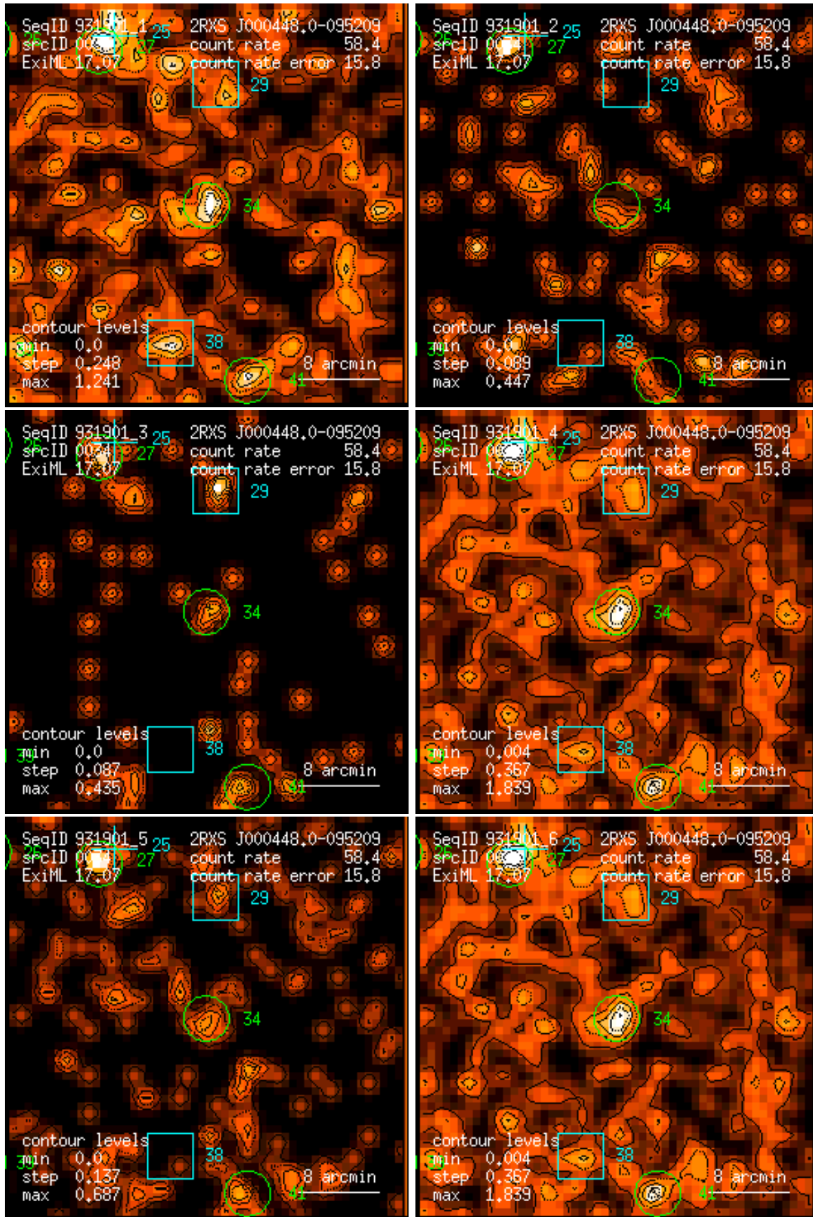
Figure 34: RASS 931901: detection 0034: band rate images, Gaussian filter: (1) PSPC channels 11 – 41, (2) 52 – 90, (3) 91 – 201, (4) 11 – 235, (5) 52 – 201, (6) 11 – 201. Broad band rates in counts/ks. Band rate contour levels in counts/ks/arcmin 2 .
