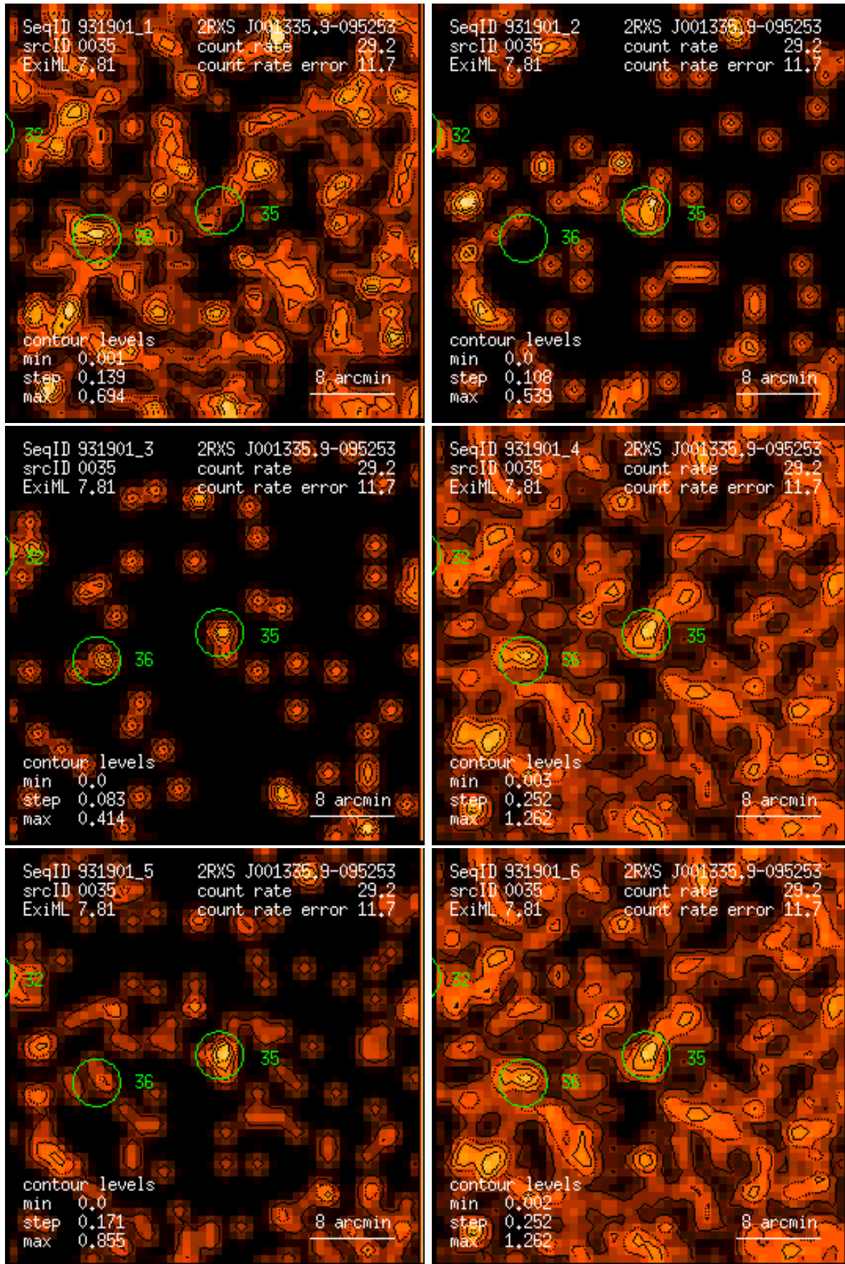
Figure 35: RASS 931901: detection 0035: band rate images, Gaussian filter: (1) PSPC channels 11 – 41, (2) 52 – 90, (3) 91 – 201, (4) 11 – 235, (5) 52 – 201, (6) 11 – 201. Broad band rates in counts/ks. Band rate contour levels in counts/ks/arcmin 2 .
