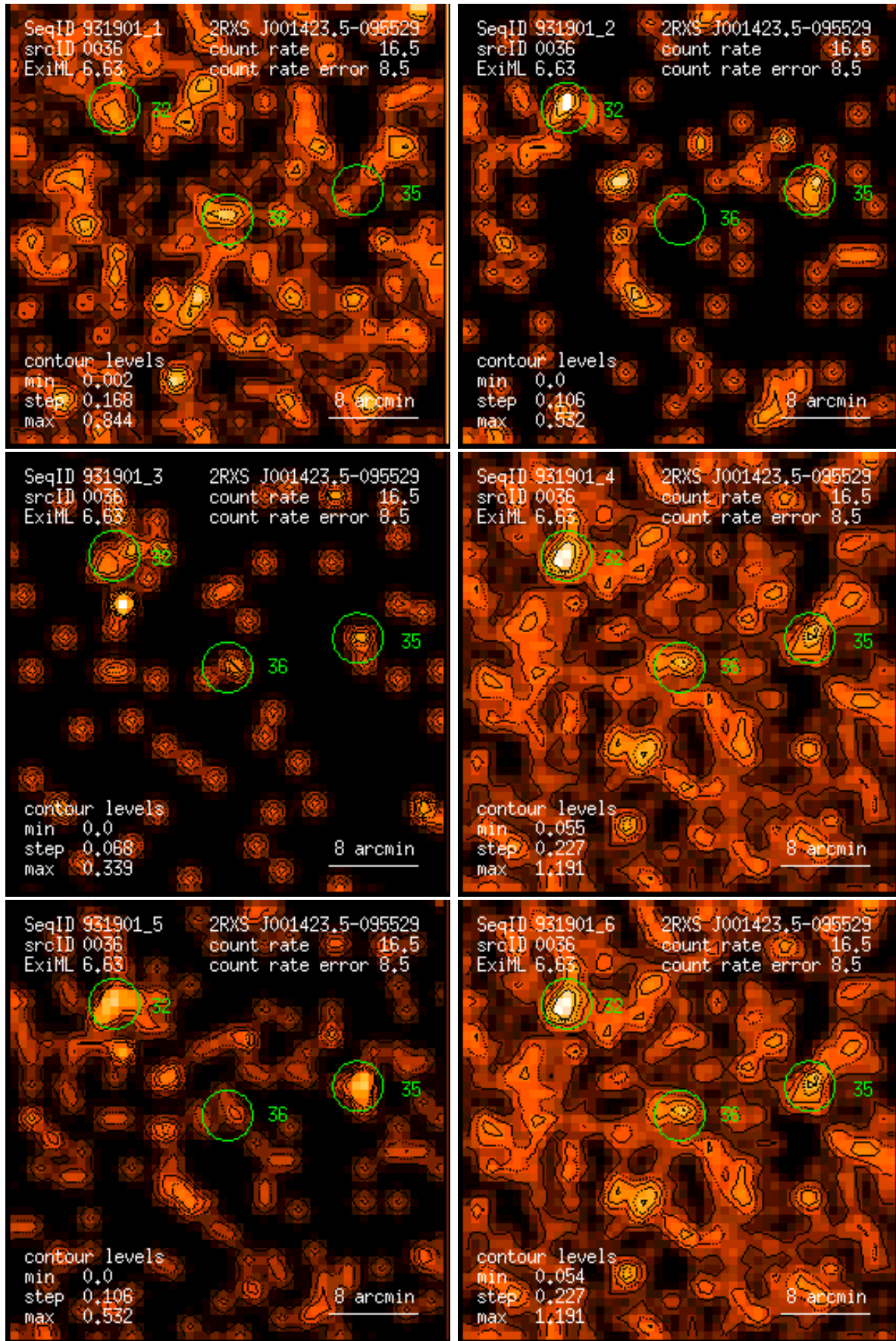
Figure 36: RASS 931901: detection 0036: band rate images, Gaussian filter: (1) PSPC channels 11 – 41, (2) 52 – 90, (3) 91 – 201, (4) 11 – 235, (5) 52 – 201, (6) 11 – 201. Broad band rates in counts/ks. Band rate contour levels in counts/ks/arcmin 2 .
