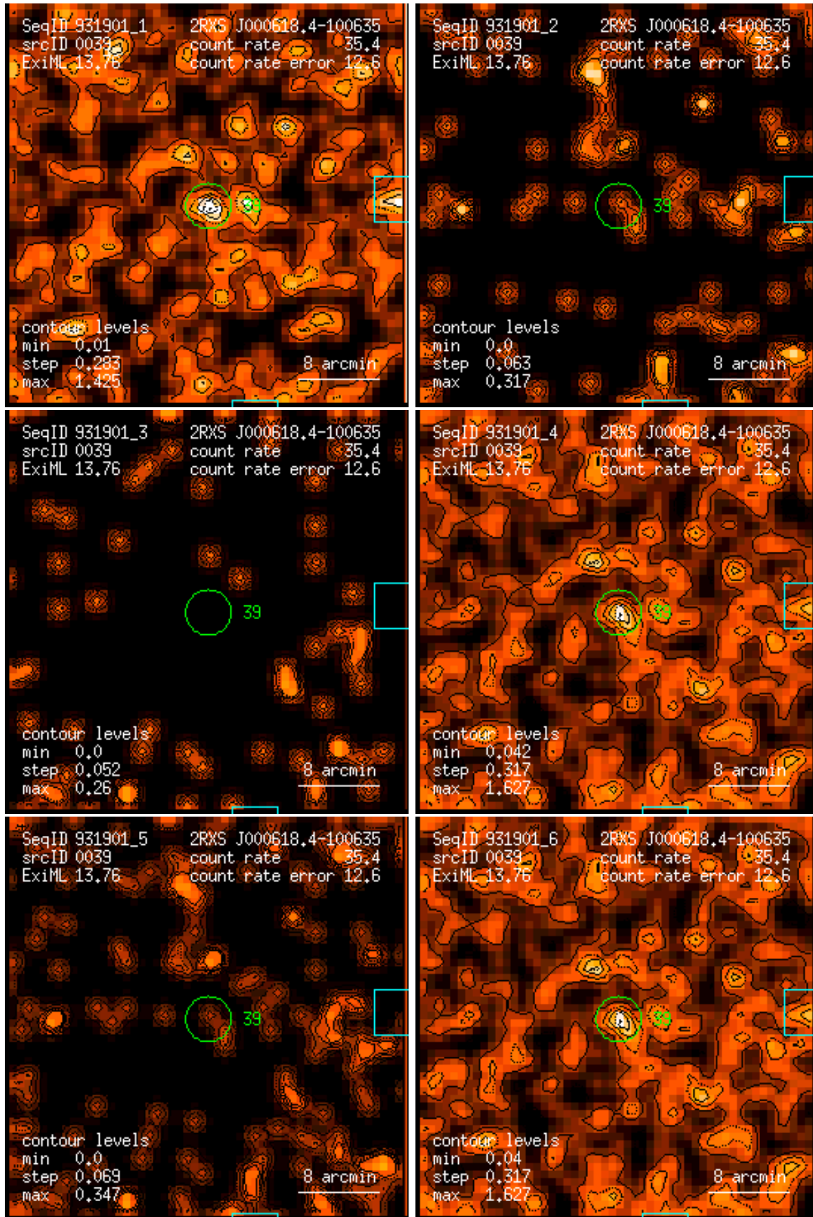
Figure 39: RASS 931901: detection 0039: band rate images, Gaussian filter: (1) PSPC channels 11 – 41, (2) 52 – 90, (3) 91 – 201, (4) 11 – 235, (5) 52 – 201, (6) 11 – 201. Broad band rates in counts/ks. Band rate contour levels in counts/ks/arcmin 2 .
