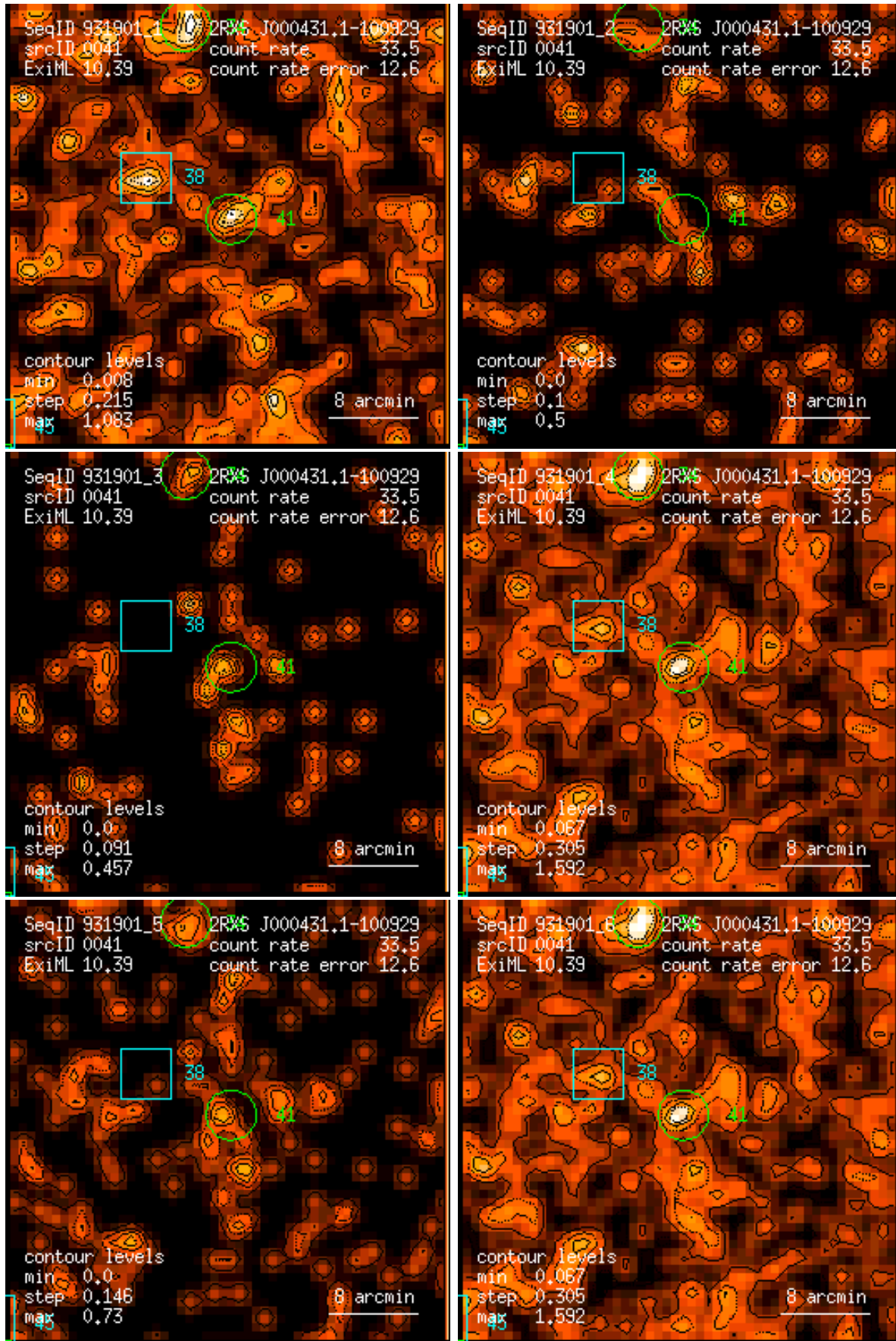
Figure 41: RASS 931901: detection 0041: band rate images, Gaussian filter: (1) PSPC channels 11 – 41, (2) 52 – 90, (3) 91 – 201, (4) 11 – 235, (5) 52 – 201, (6) 11 – 201. Broad band rates in counts/ks. Band rate contour levels in counts/ks/arcmin 2 .
