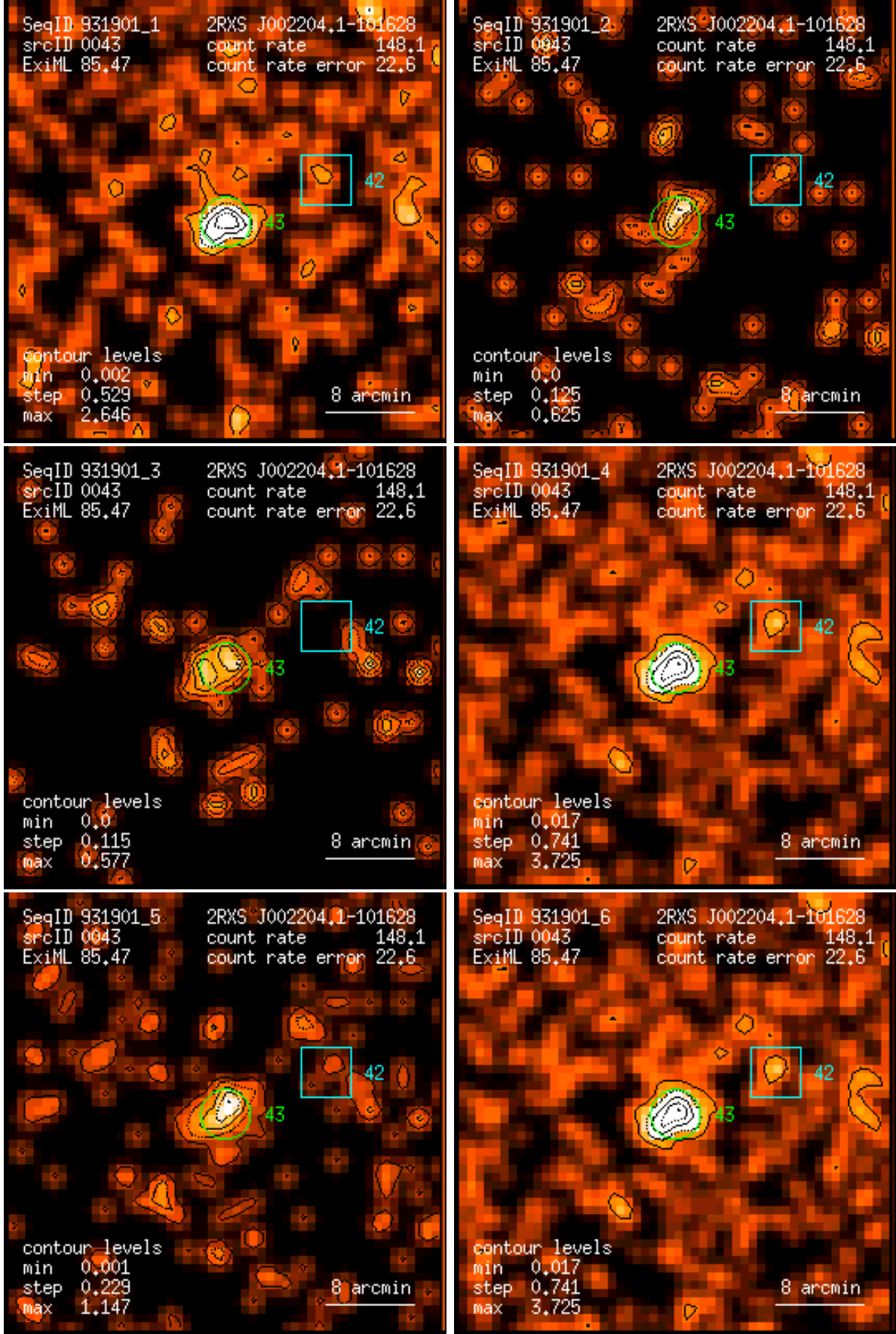
Figure 43: RASS 931901: detection 0043: band rate images, Gaussian filter: (1) PSPC channels 11 – 41, (2) 52 – 90, (3) 91 – 201, (4) 11 – 235, (5) 52 – 201, (6) 11 – 201. Broad band rates in counts/ks. Band rate contour levels in counts/ks/arcmin 2 .
