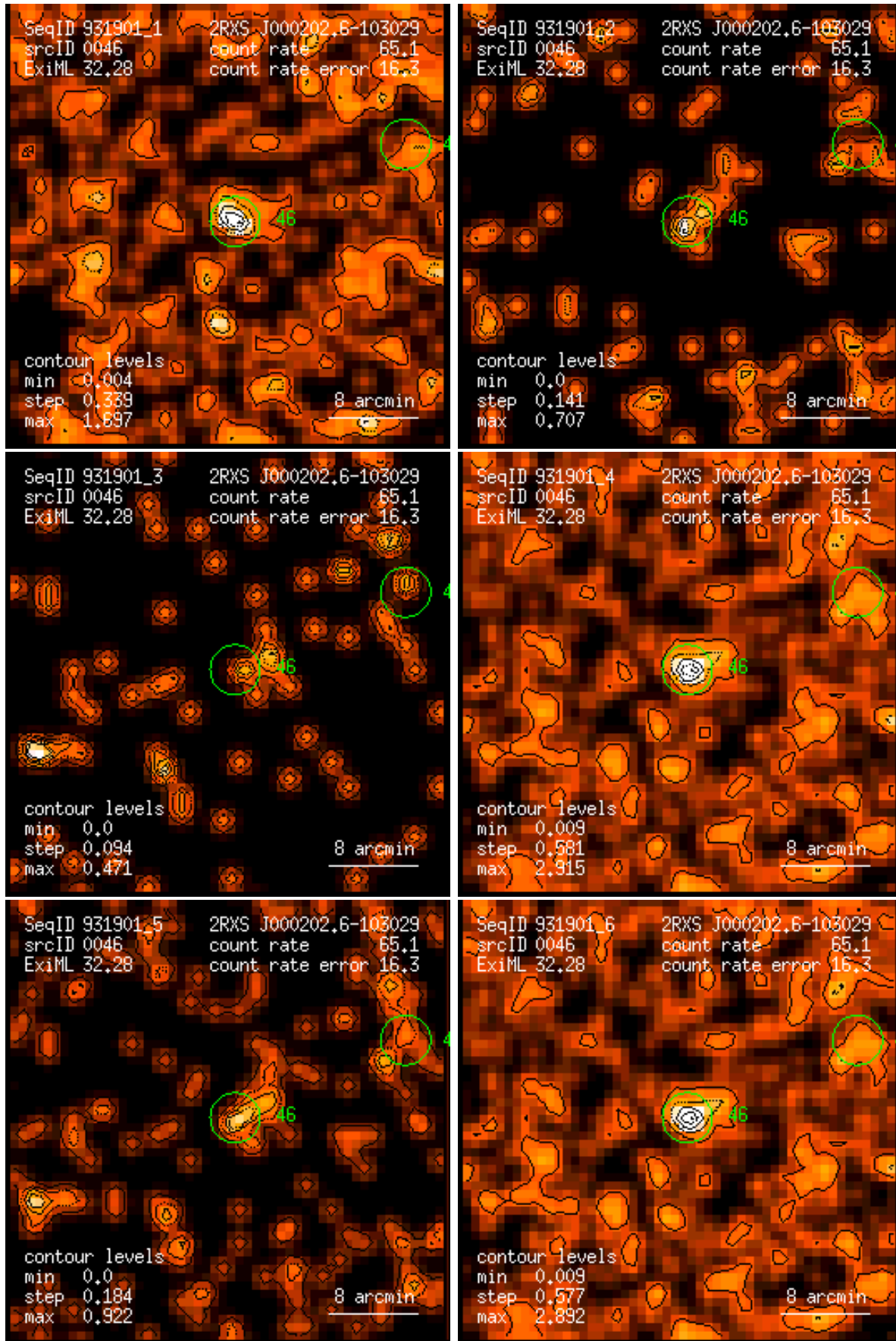
Figure 46: RASS 931901: detection 0046: band rate images, Gaussian filter: (1) PSPC channels 11 – 41, (2) 52 – 90, (3) 91 – 201, (4) 11 – 235, (5) 52 – 201, (6) 11 – 201. Broad band rates in counts/ks. Band rate contour levels in counts/ks/arcmin 2 .
