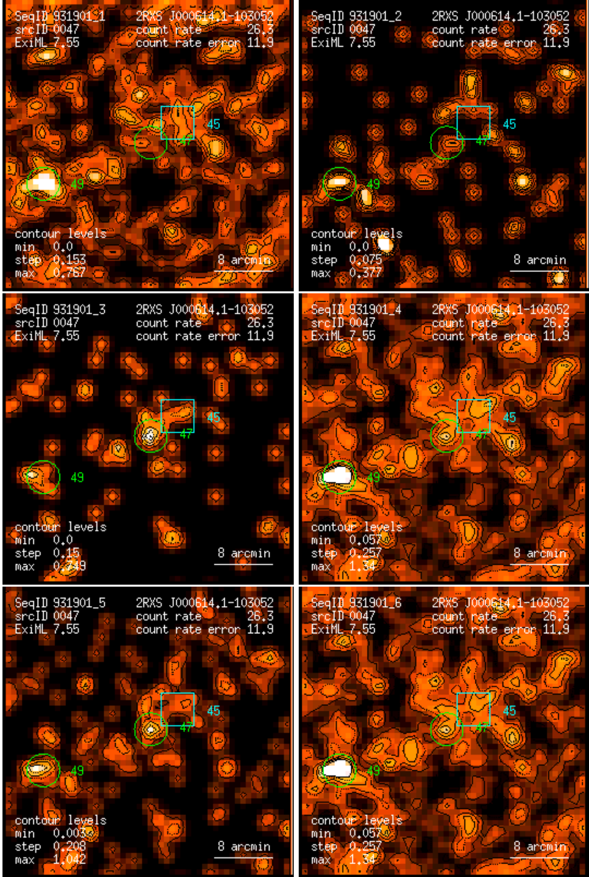
Figure 47: RASS 931901: detection 0047: band rate images, Gaussian filter: (1) PSPC channels 11 – 41, (2) 52 – 90, (3) 91 – 201, (4) 11 – 235, (5) 52 – 201, (6) 11 – 201. Broad band rates in counts/ks. Band rate contour levels in counts/ks/arcmin 2 .
