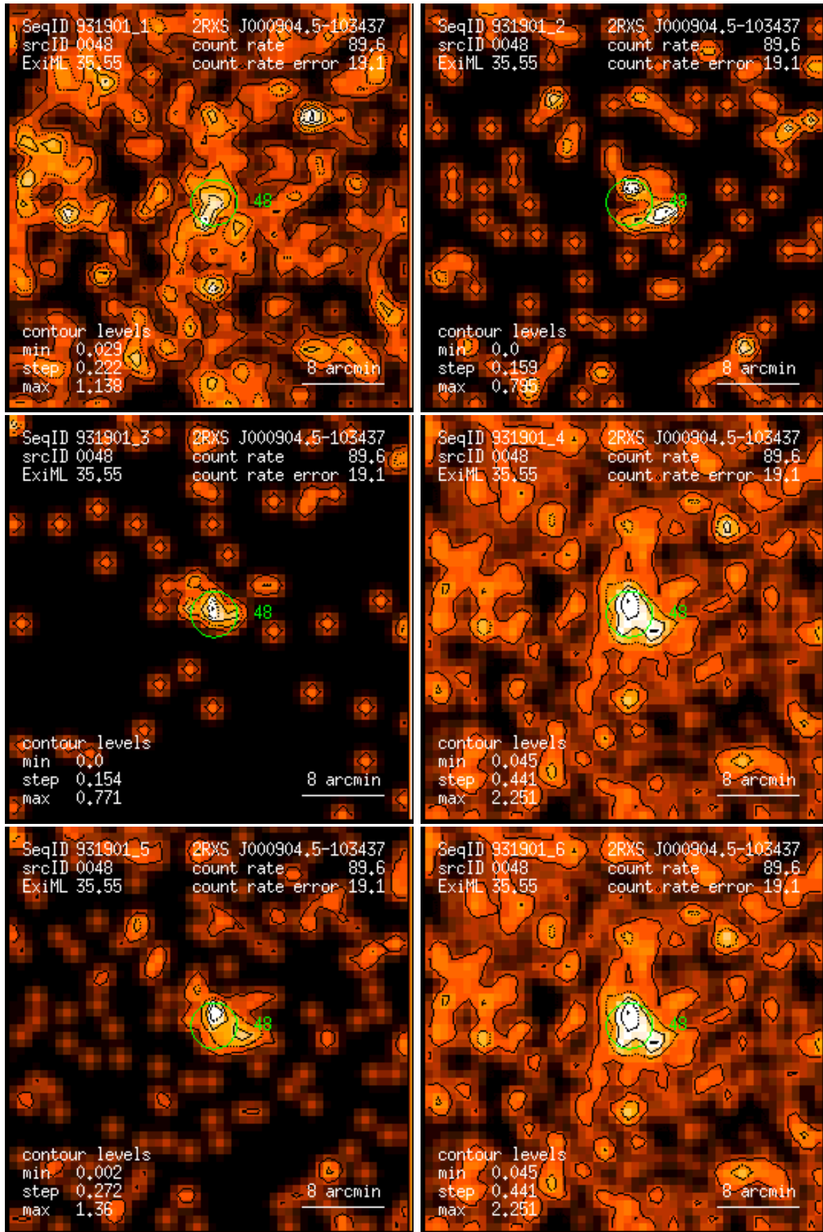
Figure 48: RASS 931901: detection 0048: band rate images, Gaussian filter: (1) PSPC channels 11 – 41, (2) 52 – 90, (3) 91 – 201, (4) 11 – 235, (5) 52 – 201, (6) 11 – 201. Broad band rates in counts/ks. Band rate contour levels in counts/ks/arcmin 2 .
