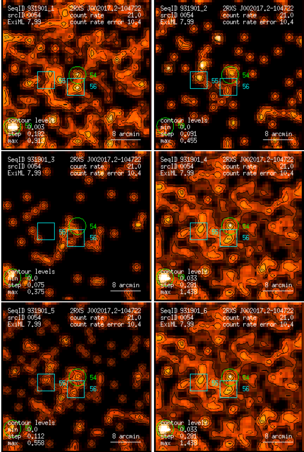
Figure 54: RASS 931901: detection 0054: band rate images, Gaussian filter: (1) PSPC channels 11 – 41, (2) 52 – 90, (3) 91 – 201, (4) 11 – 235, (5) 52 – 201, (6) 11 – 201. Broad band rates in counts/ks. Band rate contour levels in counts/ks/arcmin 2 .
