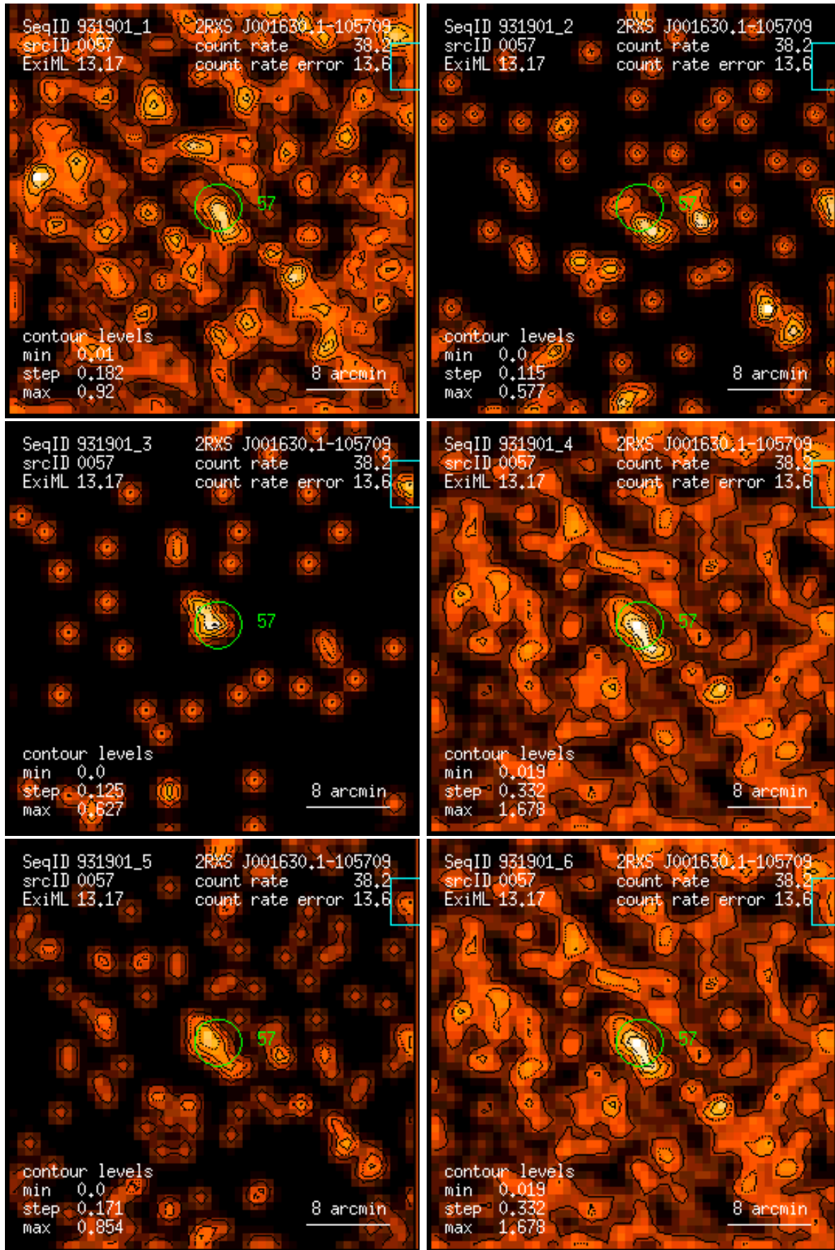
Figure 57: RASS 931901: detection 0057: band rate images, Gaussian filter: (1) PSPC channels 11 – 41, (2) 52 – 90, (3) 91 – 201, (4) 11 – 235, (5) 52 – 201, (6) 11 – 201. Broad band rates in counts/ks. Band rate contour levels in counts/ks/arcmin 2 .
