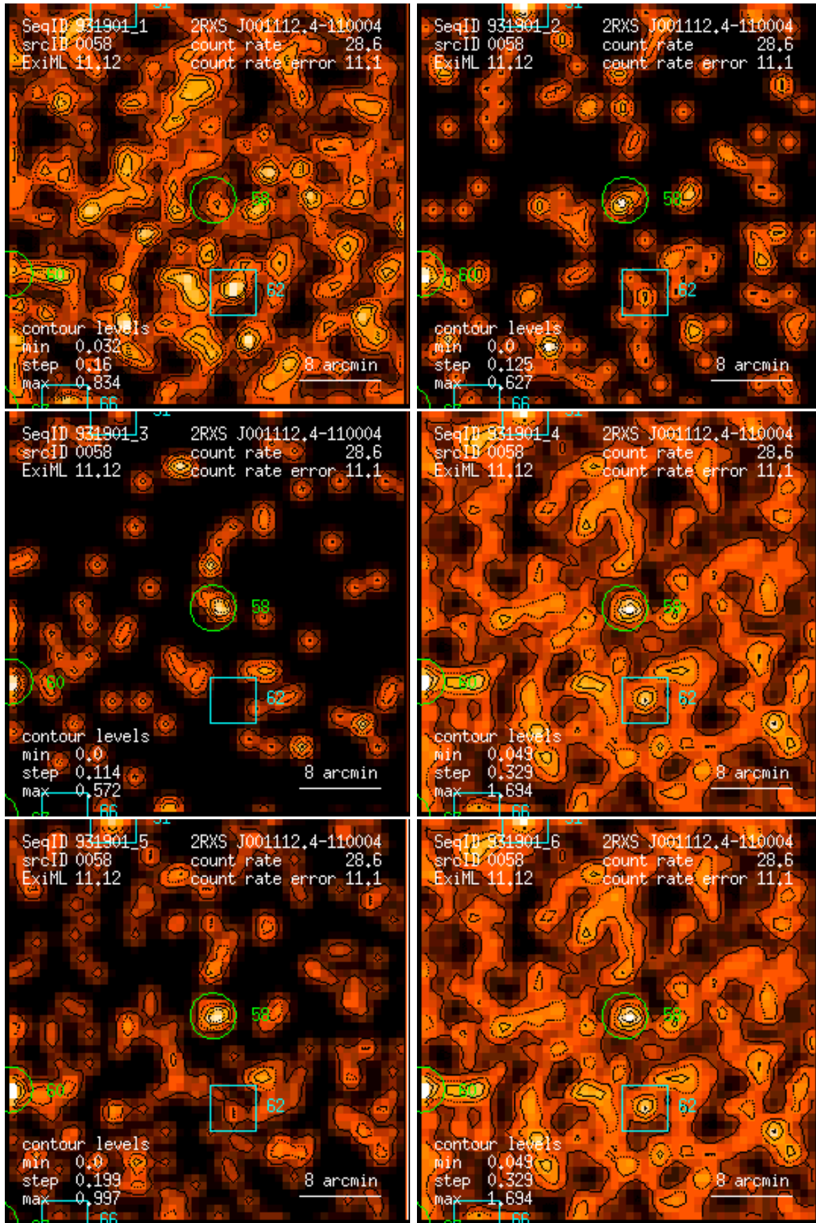
Figure 58: RASS 931901: detection 0058: band rate images, Gaussian filter: (1) PSPC channels 11 – 41, (2) 52 – 90, (3) 91 – 201, (4) 11 – 235, (5) 52 – 201, (6) 11 – 201. Broad band rates in counts/ks. Band rate contour levels in counts/ks/arcmin 2 .
