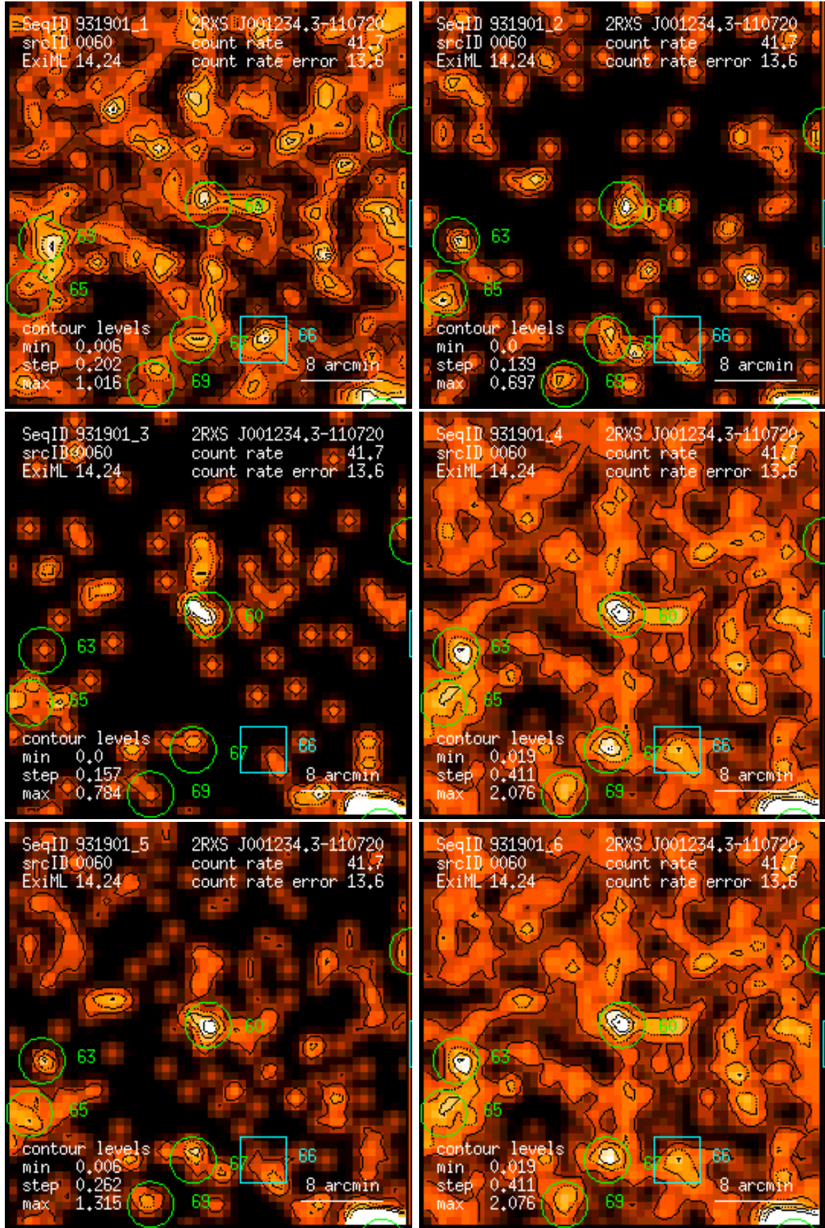
Figure 60: RASS 931901: detection 0060: band rate images, Gaussian filter: (1) PSPC channels 11 – 41, (2) 52 – 90, (3) 91 – 201, (4) 11 – 235, (5) 52 – 201, (6) 11 – 201. Broad band rates in counts/ks. Band rate contour levels in counts/ks/arcmin 2 .
