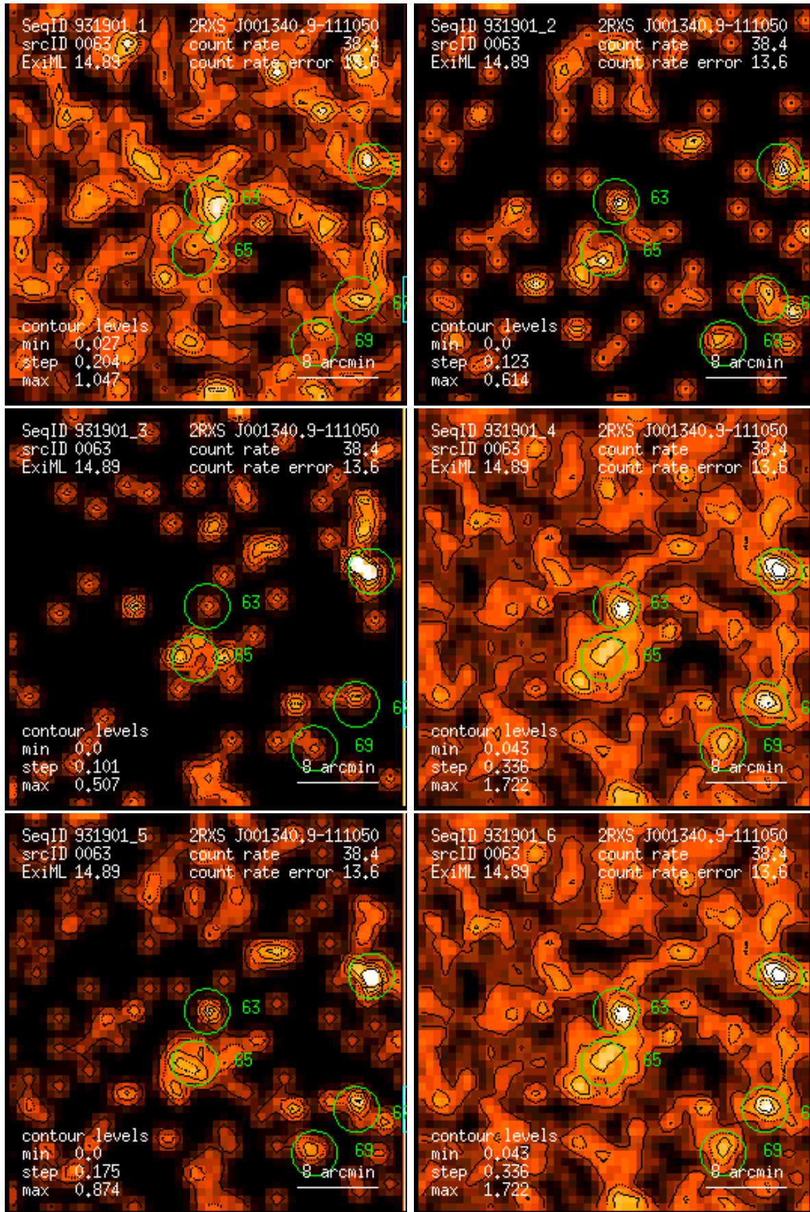
Figure 63: RASS 931901: detection 0063: band rate images, Gaussian filter: (1) PSPC channels 11 – 41, (2) 52 – 90, (3) 91 – 201, (4) 11 – 235, (5) 52 – 201, (6) 11 – 201. Broad band rates in counts/ks. Band rate contour levels in counts/ks/arcmin 2 .
