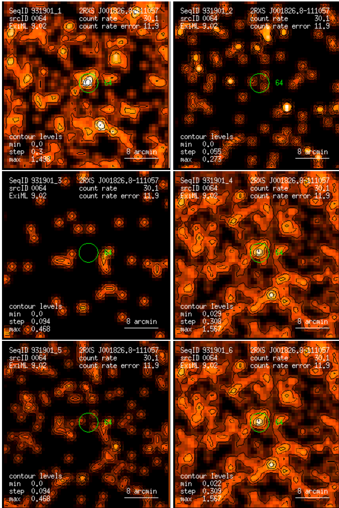
Figure 64: RASS 931901: detection 0064: band rate images, Gaussian filter: (1) PSPC channels 11 – 41, (2) 52 – 90, (3) 91 – 201, (4) 11 – 235, (5) 52 – 201, (6) 11 – 201. Broad band rates in counts/ks. Band rate contour levels in counts/ks/arcmin 2 .
