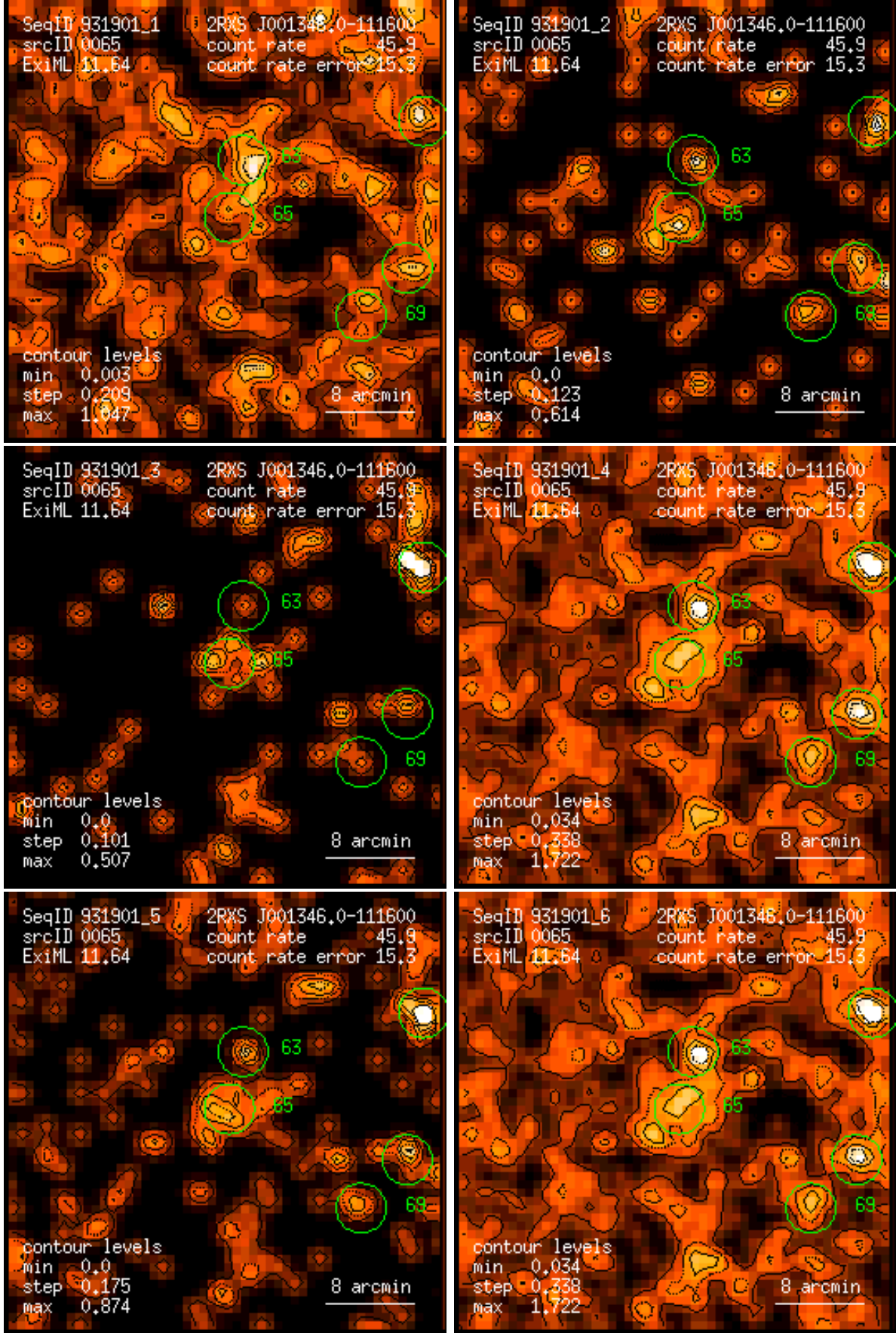
Figure 65: RASS 931901: detection 0065: band rate images, Gaussian filter: (1) PSPC channels 11 – 41, (2) 52 – 90, (3) 91 – 201, (4) 11 – 235, (5) 52 – 201, (6) 11 – 201. Broad band rates in counts/ks. Band rate contour levels in counts/ks/arcmin 2 .
