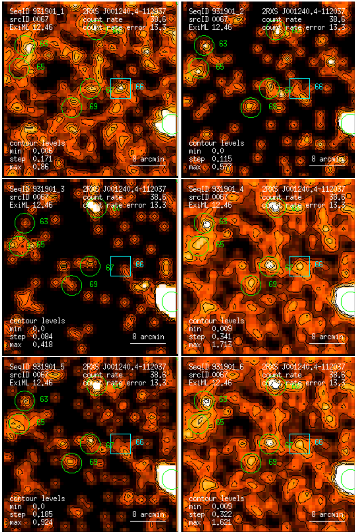
Figure 67: RASS 931901: detection 0067: band rate images, Gaussian filter: (1) PSPC channels 11 – 41, (2) 52 – 90, (3) 91 – 201, (4) 11 – 235, (5) 52 – 201, (6) 11 – 201. Broad band rates in counts/ks. Band rate contour levels in counts/ks/arcmin 2 .
