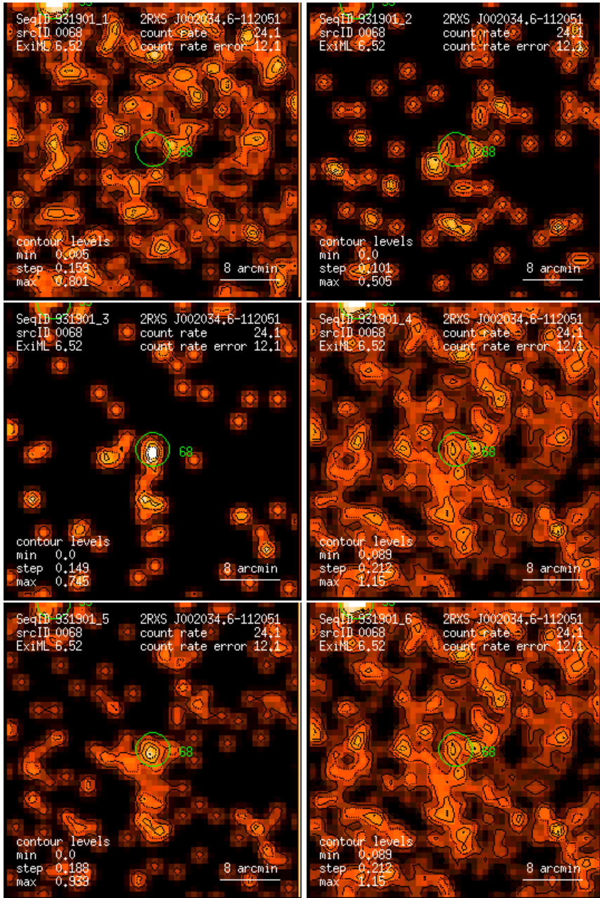
Figure 68: RASS 931901: detection 0068: band rate images, Gaussian filter: (1) PSPC channels 11 – 41, (2) 52 – 90, (3) 91 – 201, (4) 11 – 235, (5) 52 – 201, (6) 11 – 201. Broad band rates in counts/ks. Band rate contour levels in counts/ks/arcmin 2 .
