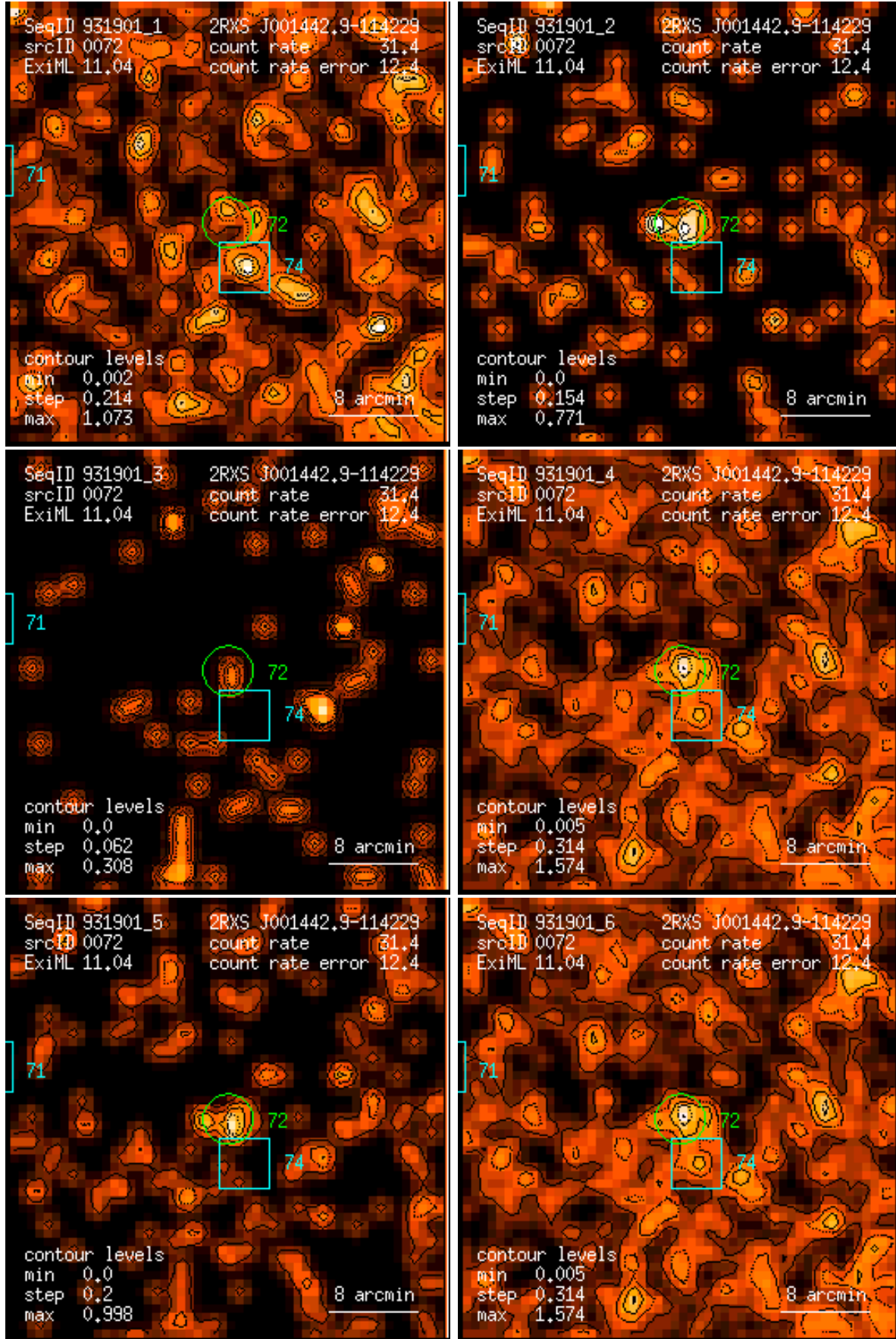
Figure 72: RASS 931901: detection 0072: band rate images, Gaussian filter: (1) PSPC channels 11 – 41, (2) 52 – 90, (3) 91 – 201, (4) 11 – 235, (5) 52 – 201, (6) 11 – 201. Broad band rates in counts/ks. Band rate contour levels in counts/ks/arcmin 2 .
