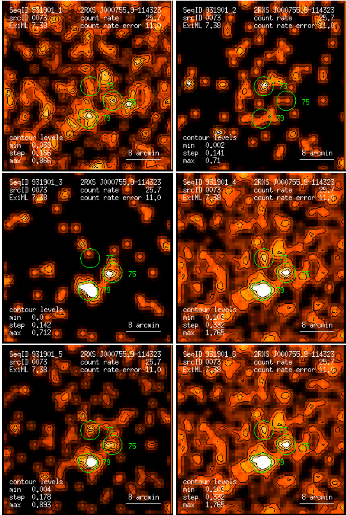
Figure 73: RASS 931901: detection 0073: band rate images, Gaussian filter: (1) PSPC channels 11 – 41, (2) 52 – 90, (3) 91 – 201, (4) 11 – 235, (5) 52 – 201, (6) 11 – 201. Broad band rates in counts/ks. Band rate contour levels in counts/ks/arcmin 2 .
