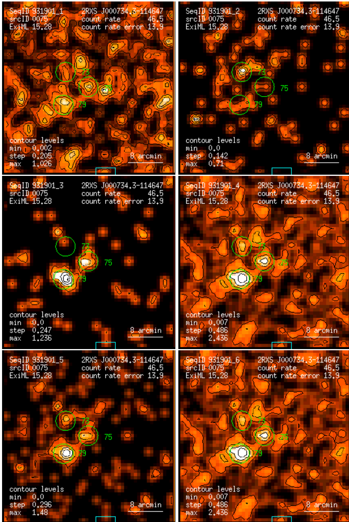
Figure 75: RASS 931901: detection 0075: band rate images, Gaussian filter: (1) PSPC channels 11 – 41, (2) 52 – 90, (3) 91 – 201, (4) 11 – 235, (5) 52 – 201, (6) 11 – 201. Broad band rates in counts/ks. Band rate contour levels in counts/ks/arcmin 2 .
