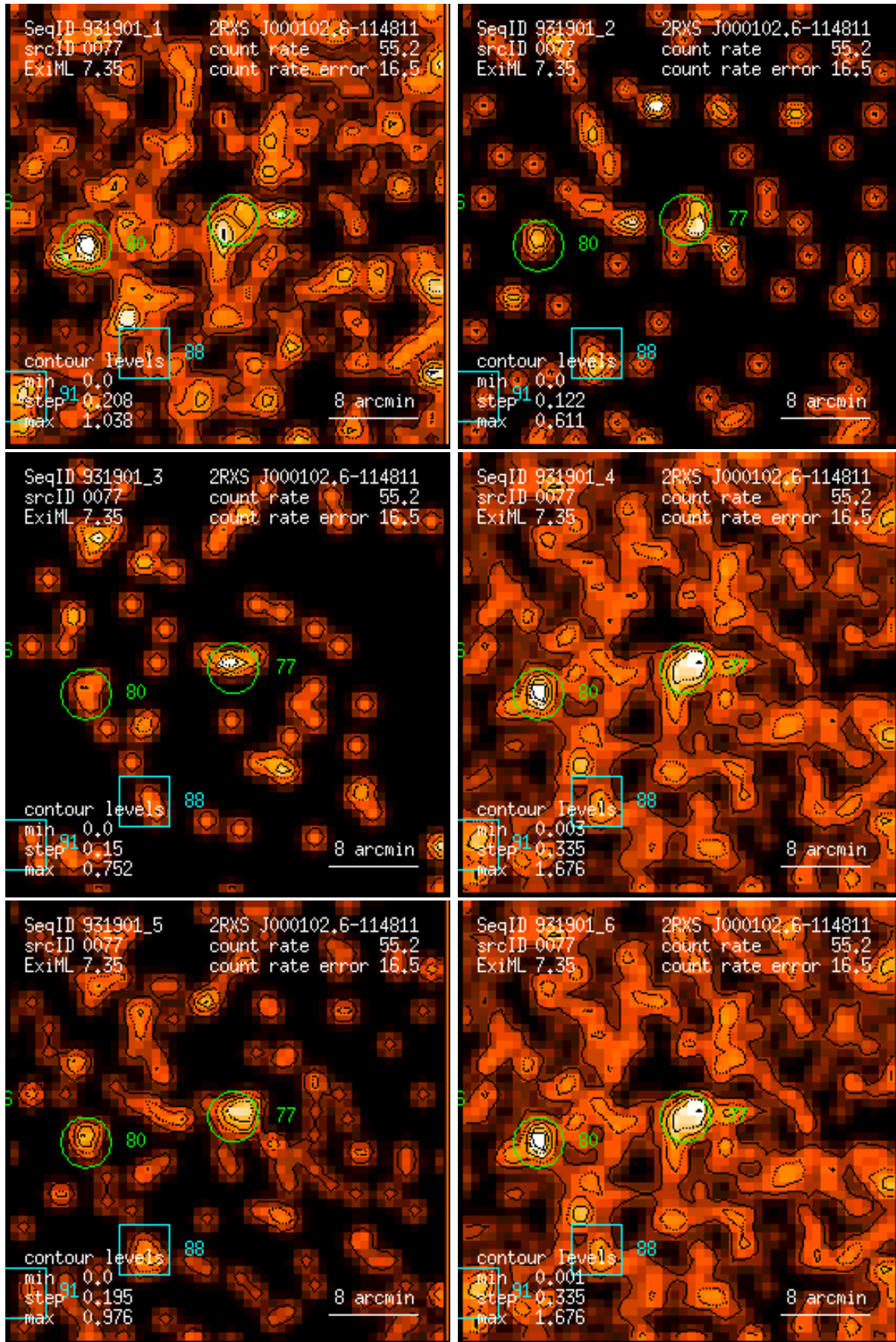
Figure 77: RASS 931901: detection 0077: band rate images, Gaussian filter: (1) PSPC channels 11 – 41, (2) 52 – 90, (3) 91 – 201, (4) 11 – 235, (5) 52 – 201, (6) 11 – 201. Broad band rates in counts/ks. Band rate contour levels in counts/ks/arcmin 2 .
