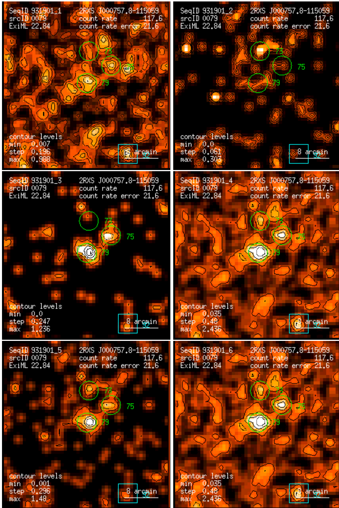
Figure 79: RASS 931901: detection 0079: band rate images, Gaussian filter: (1) PSPC channels 11 – 41, (2) 52 – 90, (3) 91 – 201, (4) 11 – 235, (5) 52 – 201, (6) 11 – 201. Broad band rates in counts/ks. Band rate contour levels in counts/ks/arcmin 2 .
