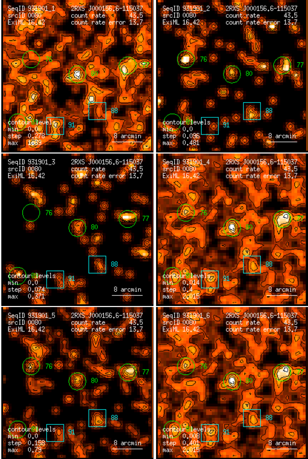
Figure 80: RASS 931901: detection 0080: band rate images, Gaussian filter: (1) PSPC channels 11 – 41, (2) 52 – 90, (3) 91 – 201, (4) 11 – 235, (5) 52 – 201, (6) 11 – 201. Broad band rates in counts/ks. Band rate contour levels in counts/ks/arcmin 2 .
