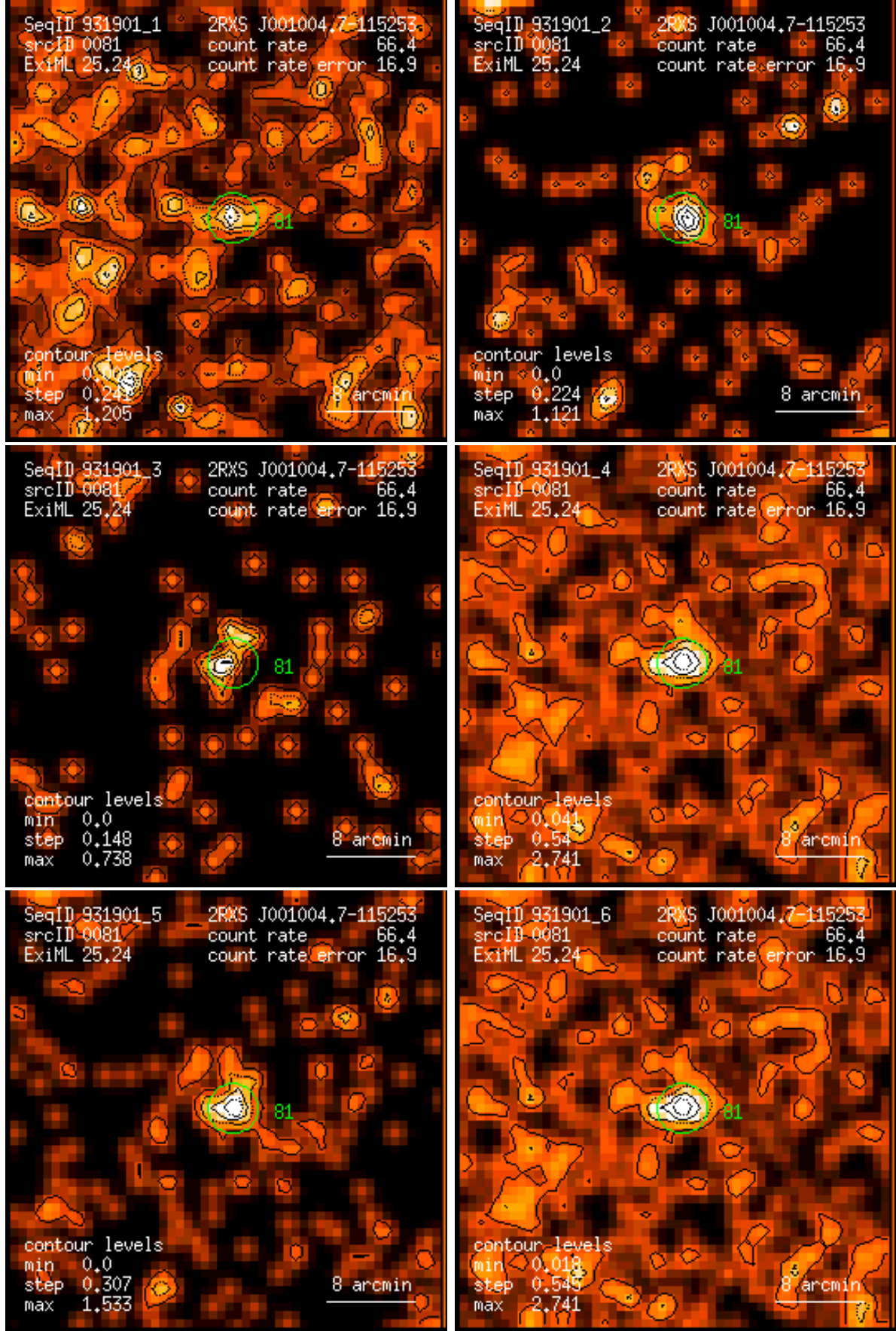
Figure 81: RASS 931901: detection 0081: band rate images, Gaussian filter: (1) PSPC channels 11 – 41, (2) 52 – 90, (3) 91 – 201, (4) 11 – 235, (5) 52 – 201, (6) 11 – 201. Broad band rates in counts/ks. Band rate contour levels in counts/ks/arcmin 2 .
