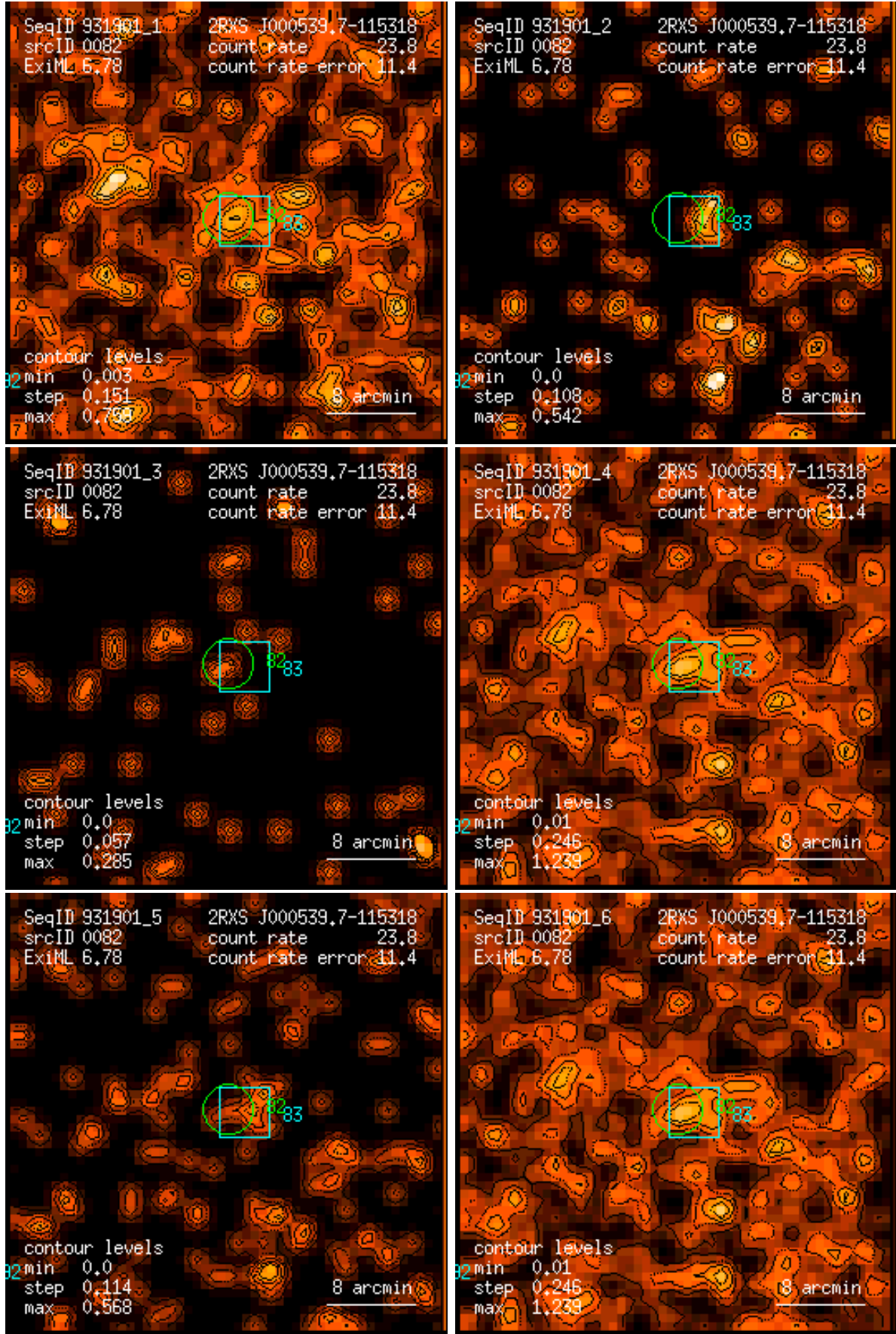
Figure 82: RASS 931901: detection 0082: band rate images, Gaussian filter: (1) PSPC channels 11 – 41, (2) 52 – 90, (3) 91 – 201, (4) 11 – 235, (5) 52 – 201, (6) 11 – 201. Broad band rates in counts/ks. Band rate contour levels in counts/ks/arcmin 2 .
