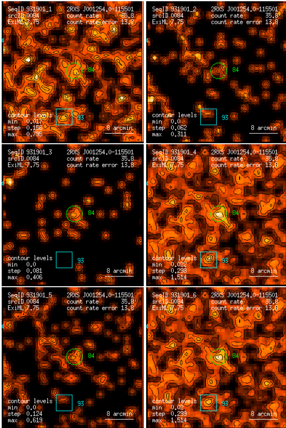
Figure 84: RASS 931901: detection 0084: band rate images, Gaussian filter: (1) PSPC channels 11 – 41, (2) 52 – 90, (3) 91 – 201, (4) 11 – 235, (5) 52 – 201, (6) 11 – 201. Broad band rates in counts/ks. Band rate contour levels in counts/ks/arcmin 2 .
