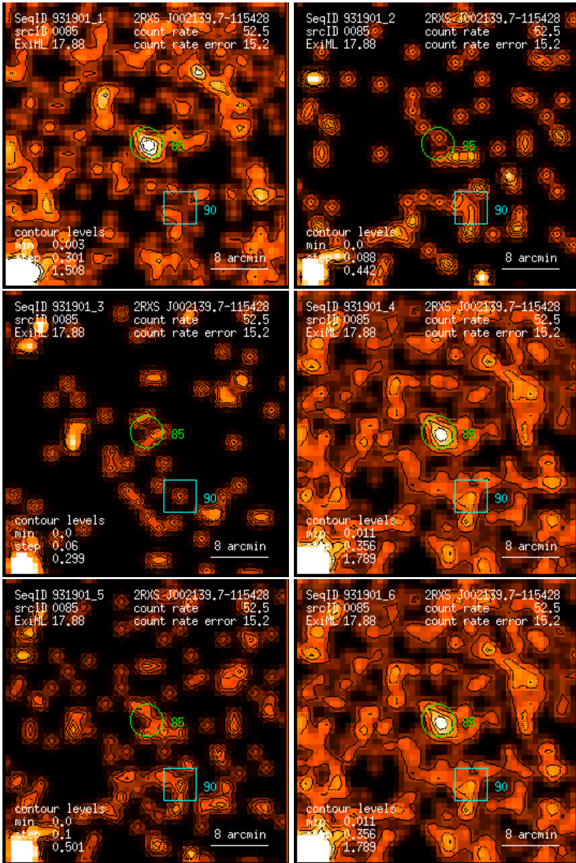
Figure 85: RASS 931901: detection 0085: band rate images, Gaussian filter: (1) PSPC channels 11 – 41, (2) 52 – 90, (3) 91 – 201, (4) 11 – 235, (5) 52 – 201, (6) 11 – 201. Broad band rates in counts/ks. Band rate contour levels in counts/ks/arcmin 2 .
