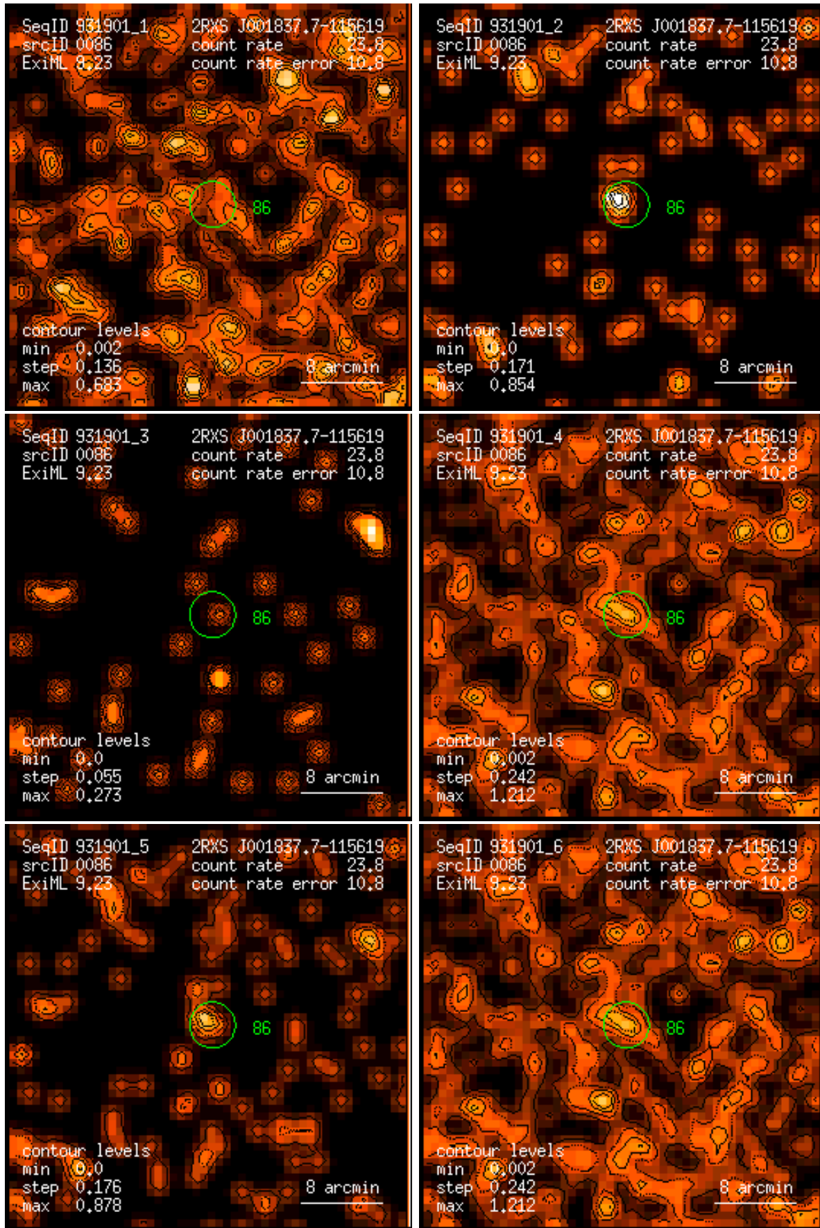
Figure 86: RASS 931901: detection 0086: band rate images, Gaussian filter: (1) PSPC channels 11 – 41, (2) 52 – 90, (3) 91 – 201, (4) 11 – 235, (5) 52 – 201, (6) 11 – 201. Broad band rates in counts/ks. Band rate contour levels in counts/ks/arcmin 2 .
