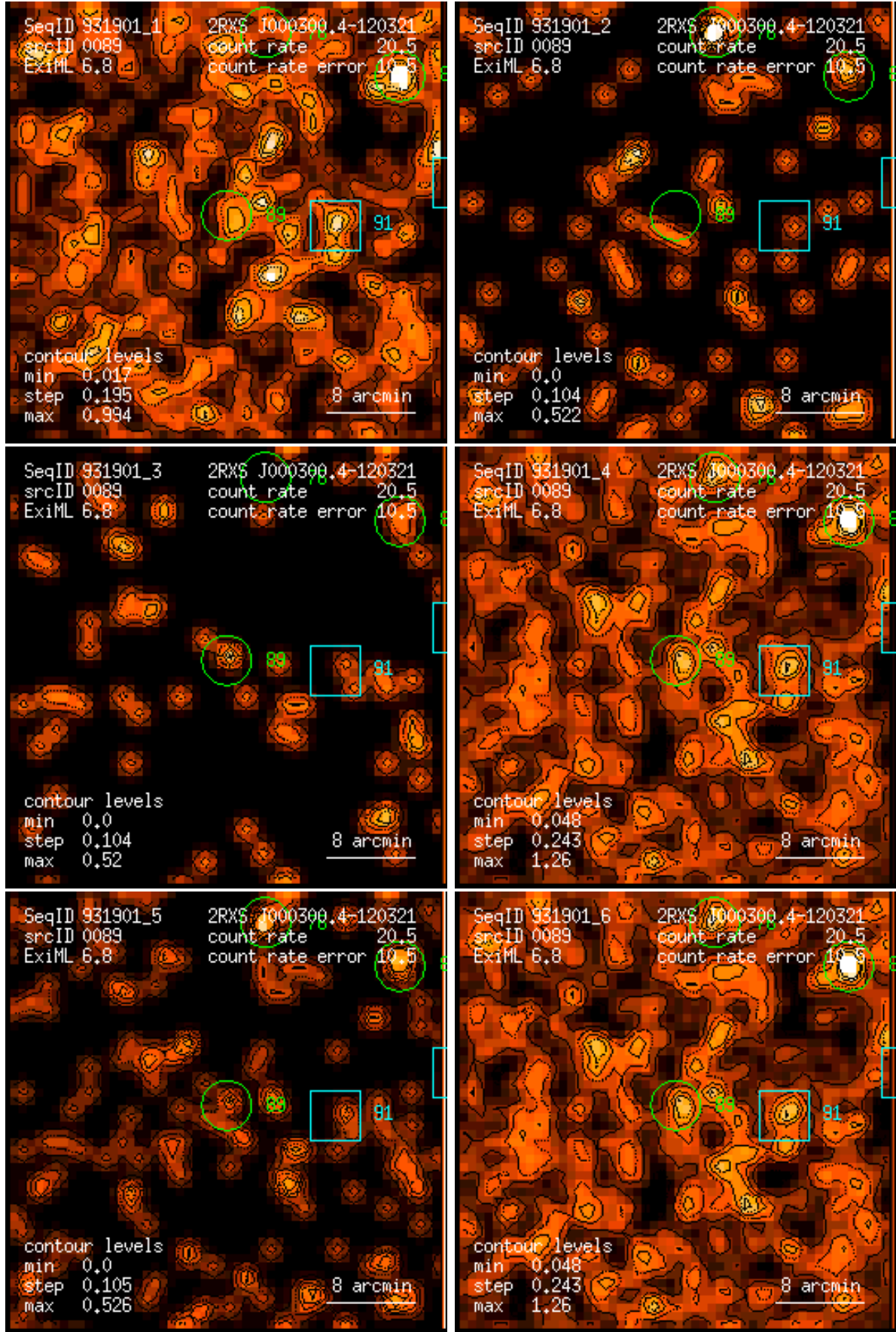
Figure 89: RASS 931901: detection 0089: band rate images, Gaussian filter: (1) PSPC channels 11 – 41, (2) 52 – 90, (3) 91 – 201, (4) 11 – 235, (5) 52 – 201, (6) 11 – 201. Broad band rates in counts/ks. Band rate contour levels in counts/ks/arcmin 2 .
