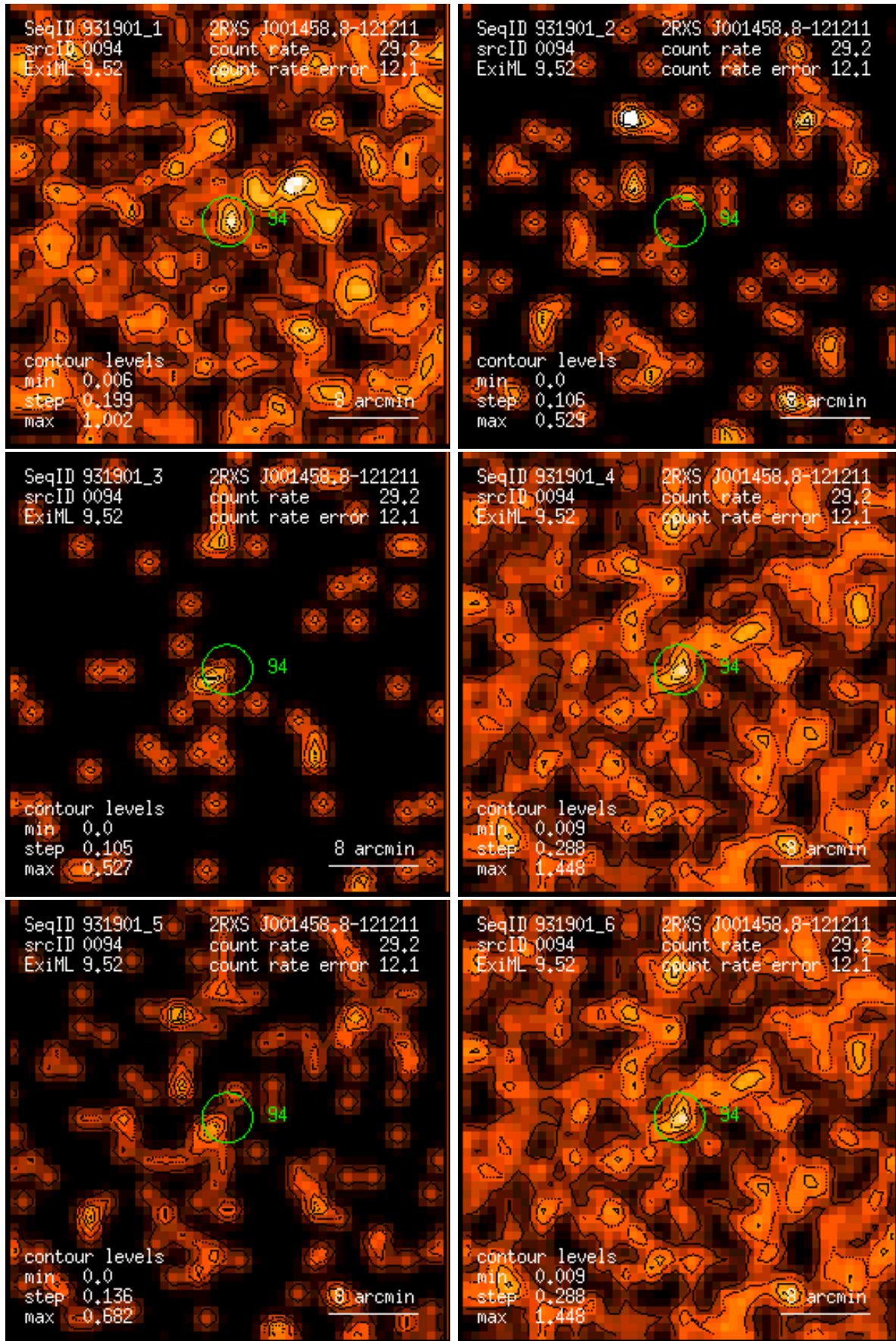
Figure 94: RASS 931901: detection 0094: band rate images, Gaussian filter: (1) PSPC channels 11 – 41, (2) 52 – 90, (3) 91 – 201, (4) 11 – 235, (5) 52 – 201, (6) 11 – 201. Broad band rates in counts/ks. Band rate contour levels in counts/ks/arcmin 2 .
