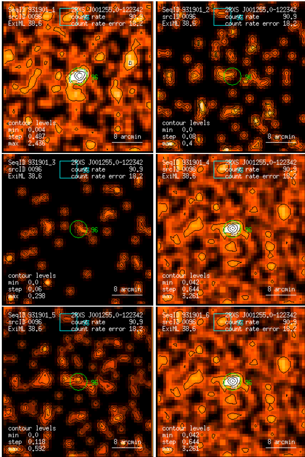
Figure 96: RASS 931901: detection 0096: band rate images, Gaussian filter: (1) PSPC channels 11 – 41, (2) 52 – 90, (3) 91 – 201, (4) 11 – 235, (5) 52 – 201, (6) 11 – 201. Broad band rates in counts/ks. Band rate contour levels in counts/ks/arcmin 2 .
