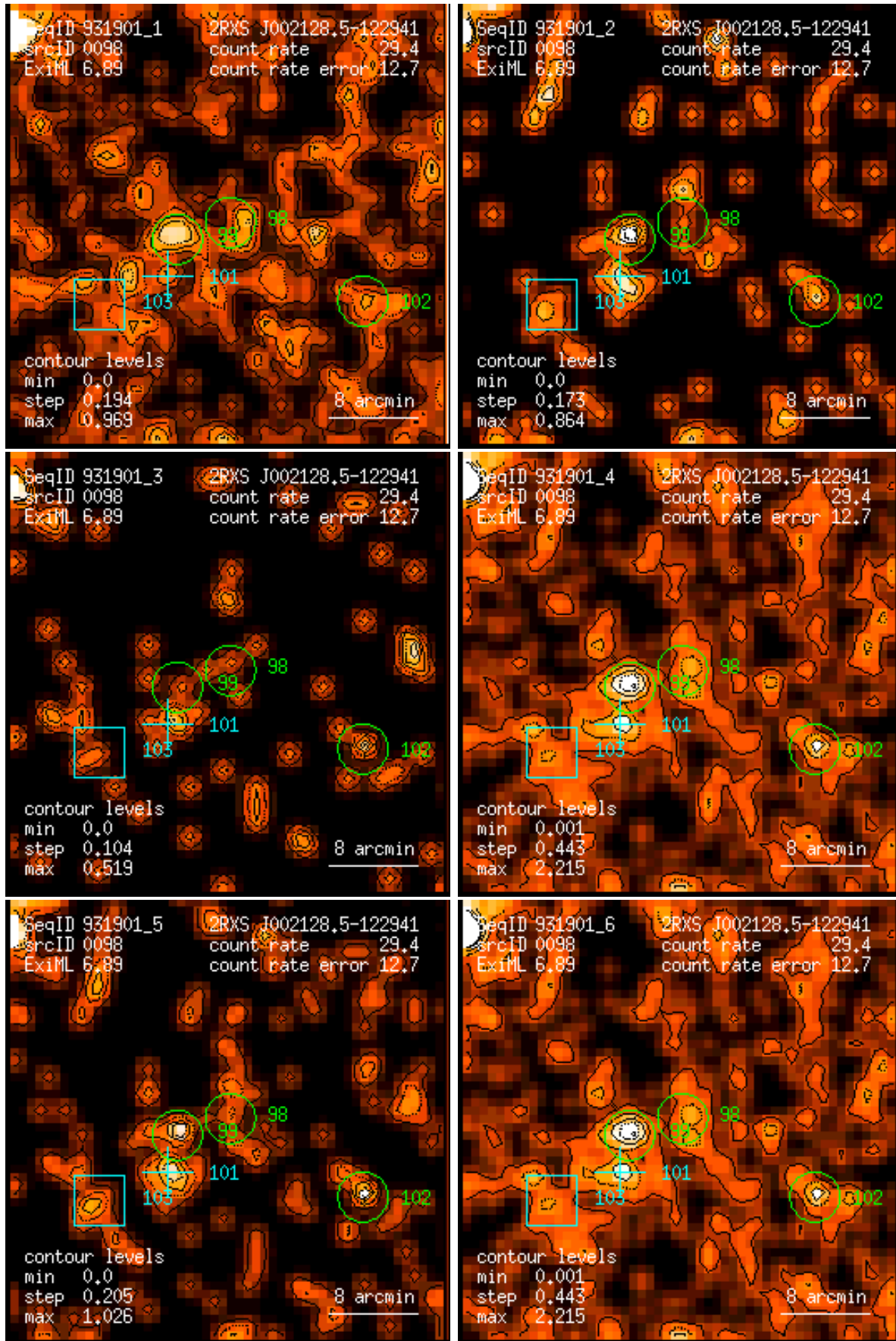
Figure 98: RASS 931901: detection 0098: band rate images, Gaussian filter: (1) PSPC channels 11 – 41, (2) 52 – 90, (3) 91 – 201, (4) 11 – 235, (5) 52 – 201, (6) 11 – 201. Broad band rates in counts/ks. Band rate contour levels in counts/ks/arcmin 2 .
