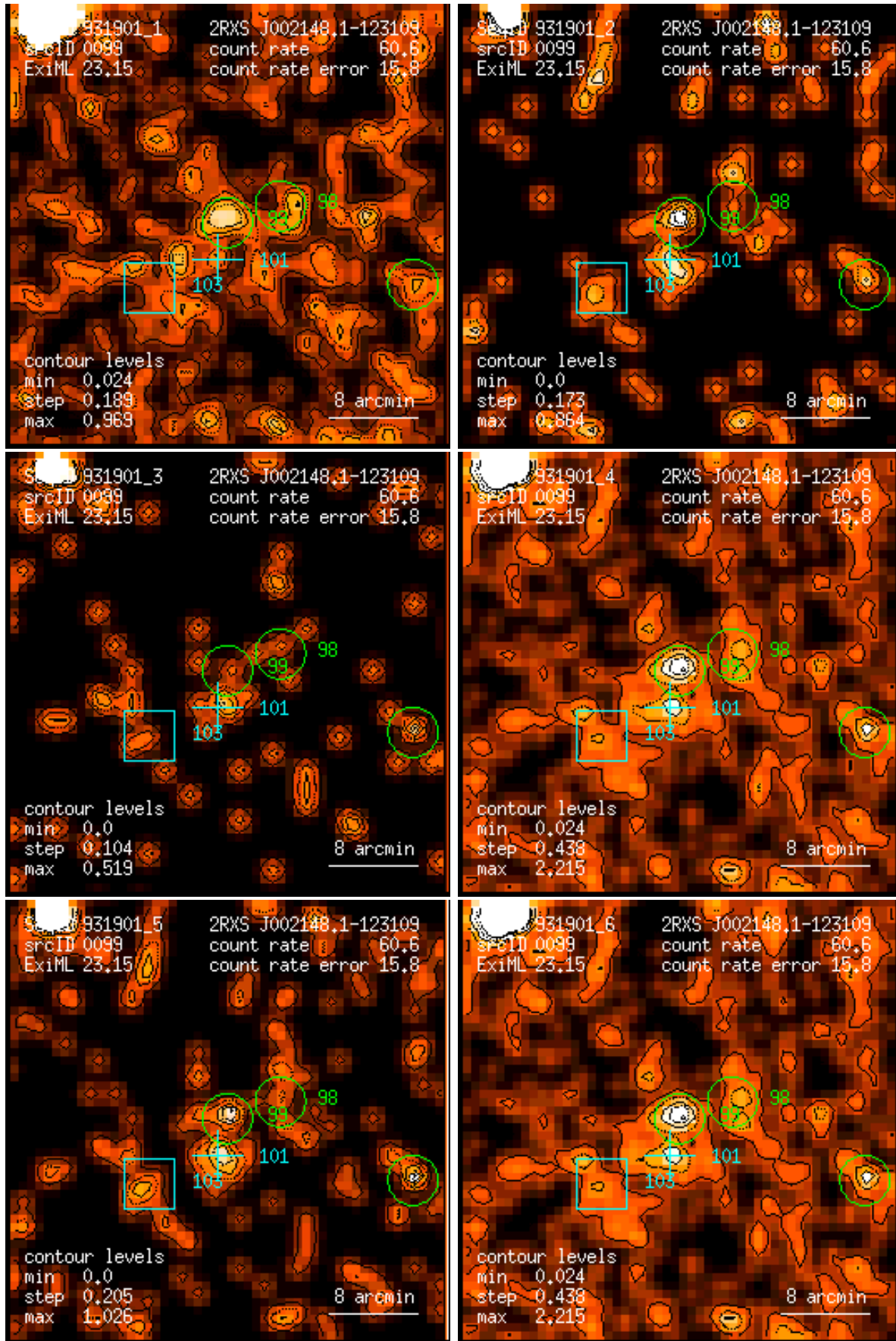
Figure 99: RASS 931901: detection 0099: band rate images, Gaussian filter: (1) PSPC channels 11 – 41, (2) 52 – 90, (3) 91 – 201, (4) 11 – 235, (5) 52 – 201, (6) 11 – 201. Broad band rates in counts/ks. Band rate contour levels in counts/ks/arcmin 2 .
