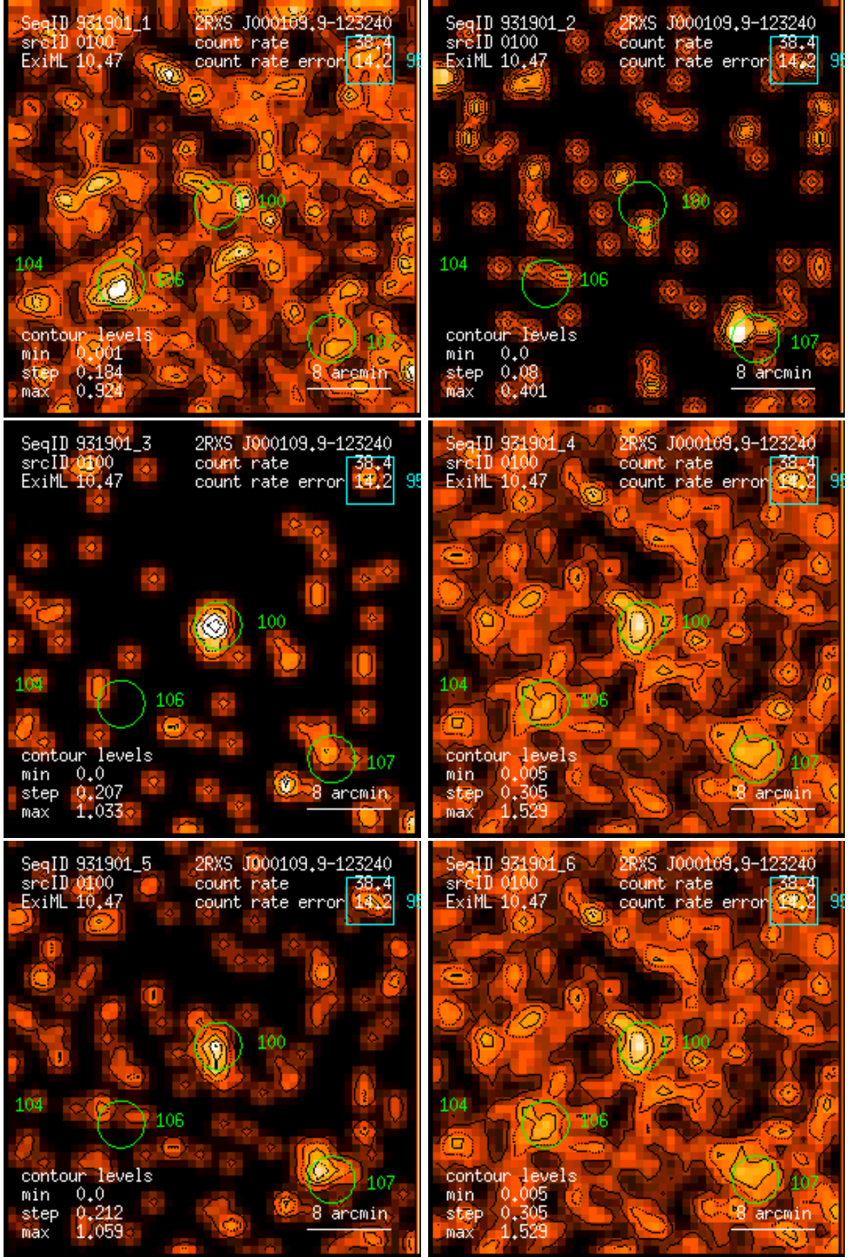
Figure 100: RASS 931901: detection 0100: band rate images, Gaussian filter: (1) PSPC channels 11 – 41, (2) 52 – 90, (3) 91 – 201, (4) 11 – 235, (5) 52 – 201, (6) 11 – 201. Broad band rates in counts/ks. Band rate contour levels in counts/ks/arcmin 2 .
