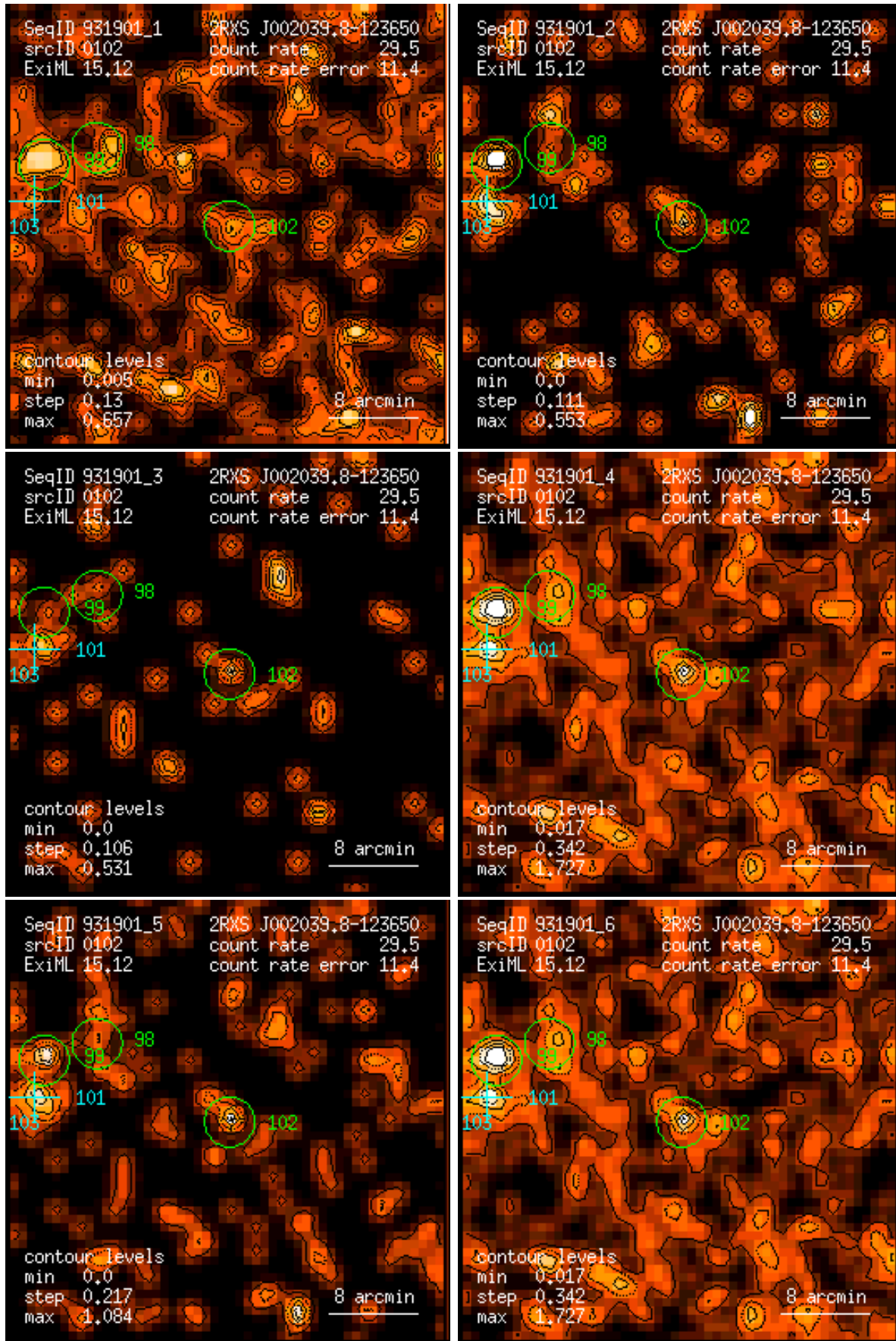
Figure 102: RASS 931901: detection 0102: band rate images, Gaussian filter: (1) PSPC channels 11 – 41, (2) 52 – 90, (3) 91 – 201, (4) 11 – 235, (5) 52 – 201, (6) 11 – 201. Broad band rates in counts/ks. Band rate contour levels in counts/ks/arcmin 2 .
